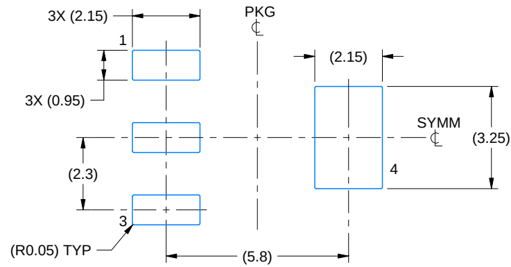
LAND PATTERN EXAMPLE EXPOSED METAL SHOWN SCALE:6X
