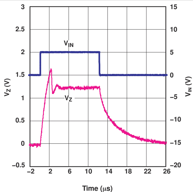
图 5-3. Start-Up Characteristics
