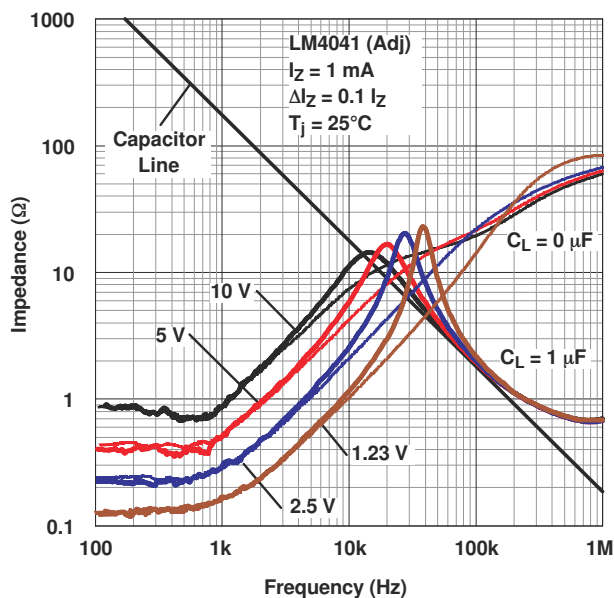
FIG 5-7. Output Impedance vs Frequency
