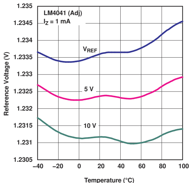
FIG 5-5. Reference Voltage vs Temperature (for Different Reverse Voltages)
