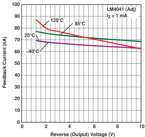
FIG 5-6. Feedback Current vs Reverse (Output) Voltage (for Different Temperatures)
