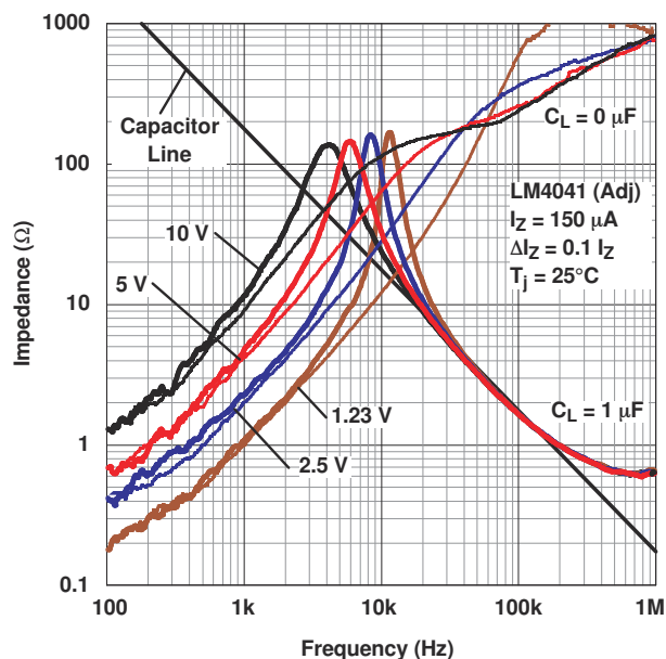
FIG 5-8. Output Impedance vs Frequency
