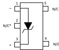
✎ 4-2. DCK Package 5-Pin SC70 Top View
