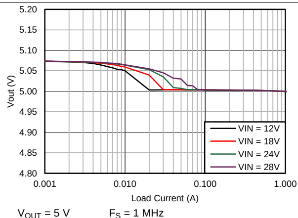
Figure 10. V_{OUT} Regulation
