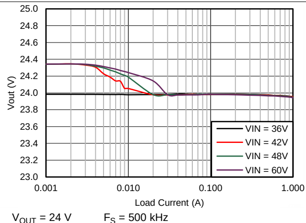
Figure 12. V_{OUT} Regulation
