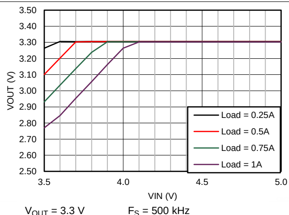
Figure 50. Dropout Curve
