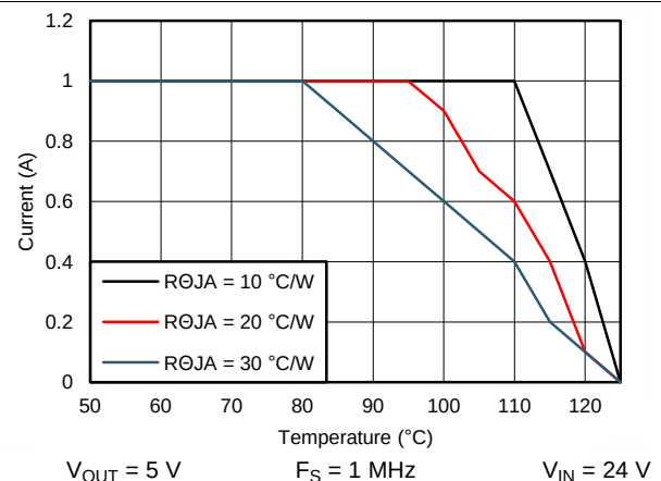
Figure 70. Derating Curve
