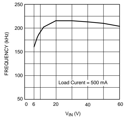
Figure 17. Frequency vs V_{IN}
