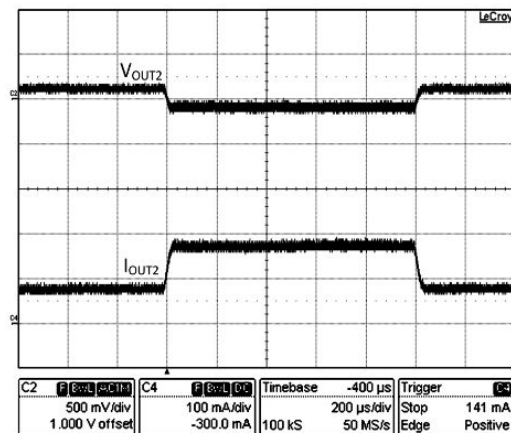
FIG 8-11. Step Load Response (VIN = 48 V, IOUT1 = 0, Step Load on IOUT2 = 80 mA to 180 mA)
