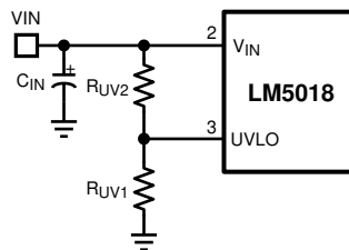
FIG 7-2. UVLO Resistor Setting
