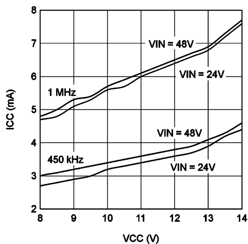
6-4. I_{CC} versus External V_{CC}
