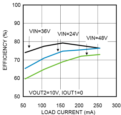
FIG 8-9. Efficiency at 750 kHz, VOUT1 = 10 V
