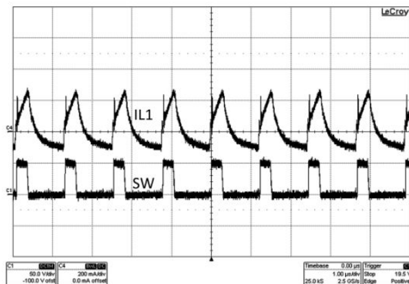
FIG 8-10. Steady-State Waveform (VIN = 48 V, IOUT1 = 0 mA, IOUT2 = 100 mA)
