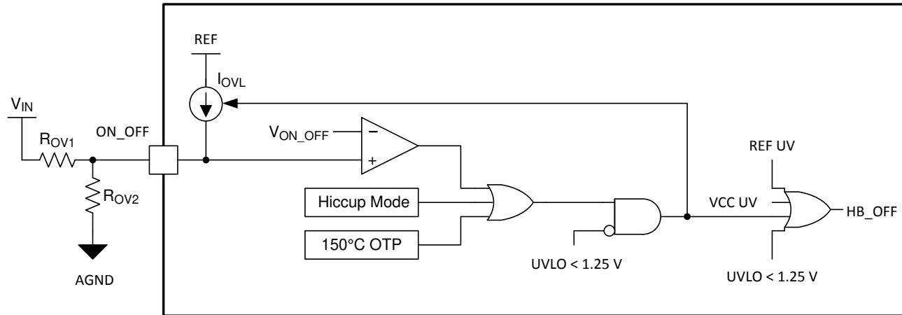
FIG 7-21. ON/OFF Pin Configured as OVP Pin
