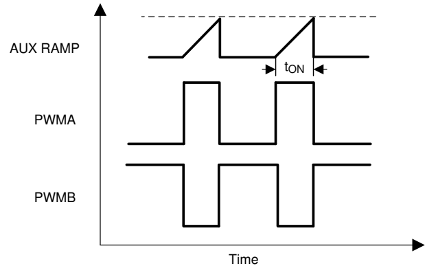
FIG 7-24. Constant On-Time Control Waveform
