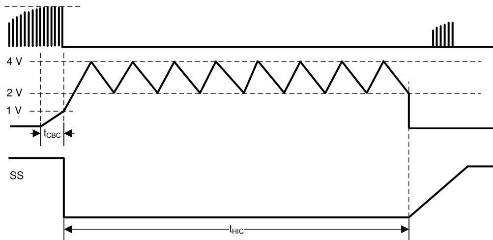
図 7-18. Hiccup Mode Activated By Continuous CBC Operation
