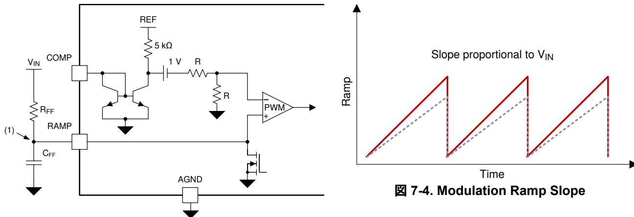
7-3. Feed-Forward Voltage-Mode Control Configuration
