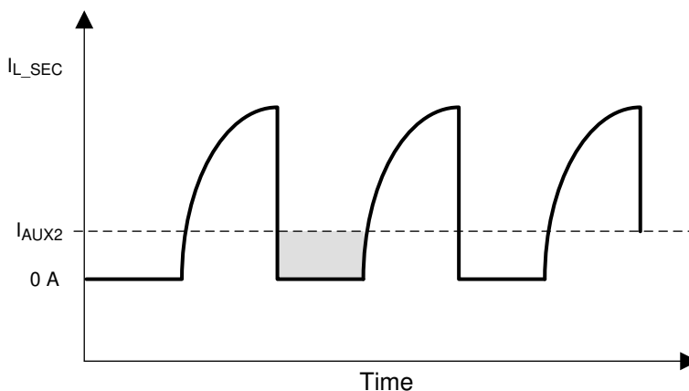
図 8-11. Auxiliary Transformer Secondary Winding Current Waveforms for C_{AUX2} Ripple Calculation
