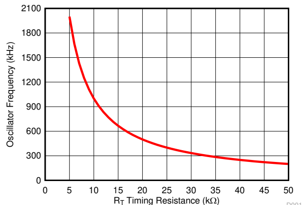
6-5. Oscillator Frequency vs R_T Timing Resistance
