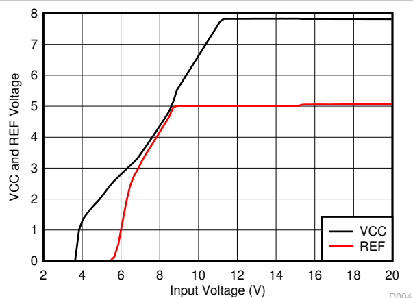
6-4. VCC and REF Voltage vs Input Voltage
