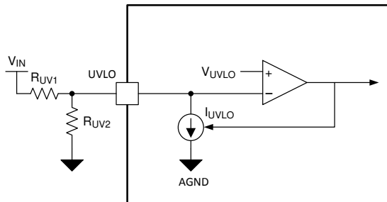
✎ 8-5. UVLO Configuration
