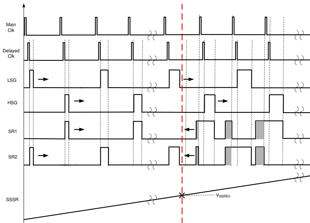
FIG 7-10. PWM Timing During Startup Process
