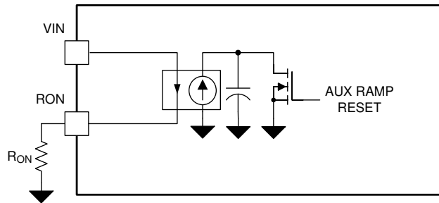
FIG 7-23. On-Time Generator
