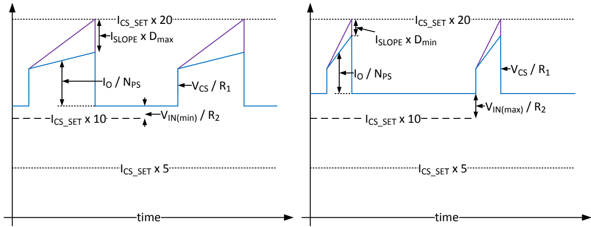
FIG 7-13. Current Sense and Current Limit Waveforms
