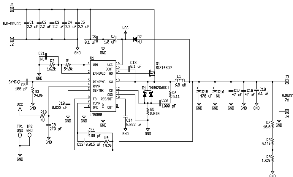
9-2. LM5088-2 Application Schematic
