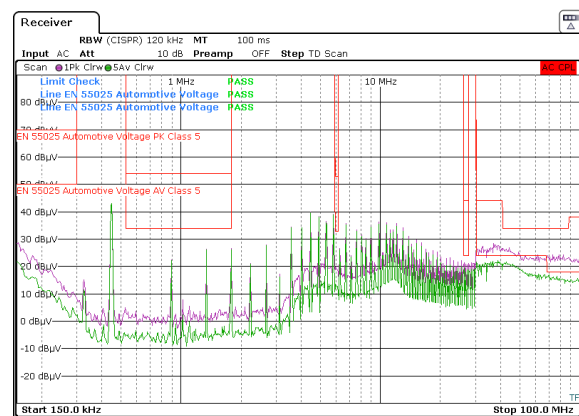
V_{IN} = 12V V_{EN2} = 0V I_{OUT1} = 10A
