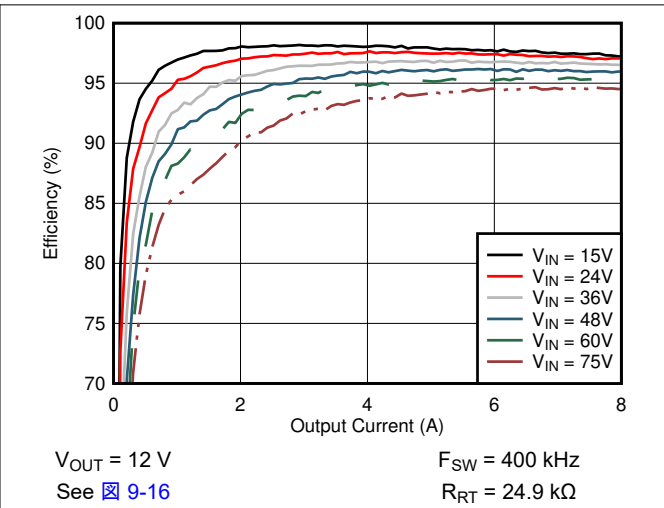
7-2. Efficiency vs Load, CCM
