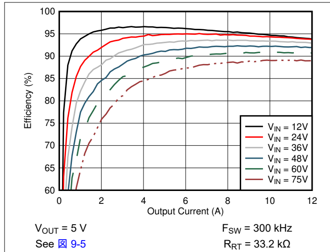
7-1. Efficiency vs Load, CCM
