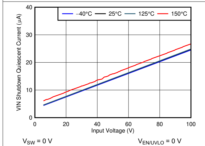
7-5. I_{Q-SHD} vs Input Voltage
