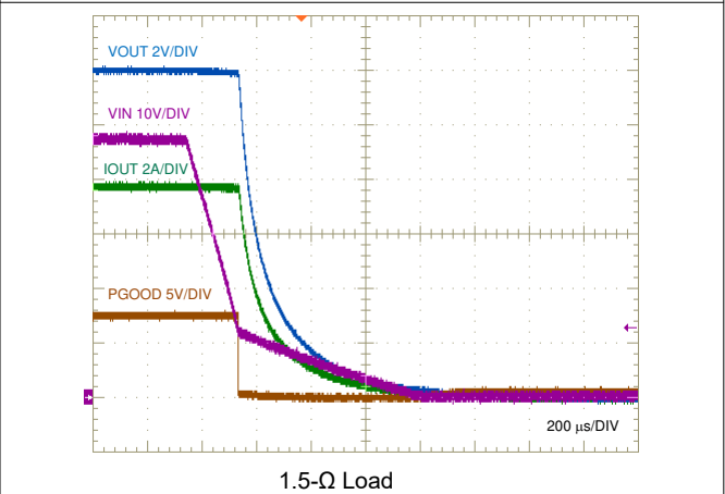
图 9-20. Shutdown By Input UVLO, 8-A Resistive Load
