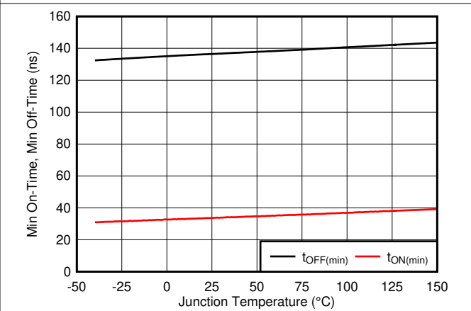
7-4. t_{ON(min)} and t_{OFF(min)} vs Junction Temperature
