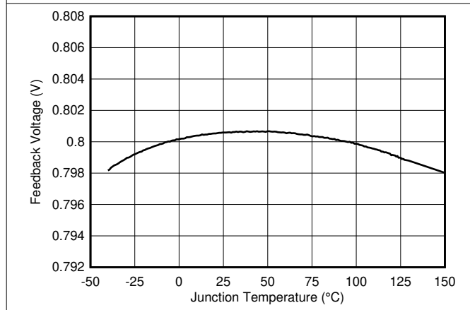
7-3. FB Voltage vs Junction Temperature
