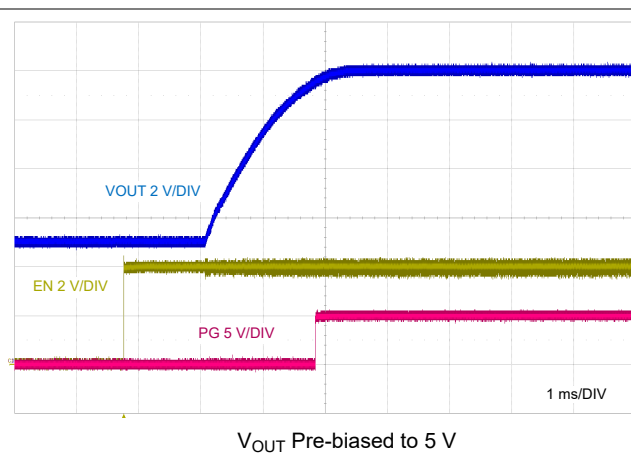
图 9-26. EN Start-Up Pre-bias Characteristic
