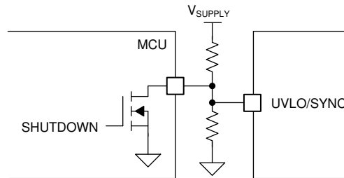
9-11. UVLO and Shutdown
