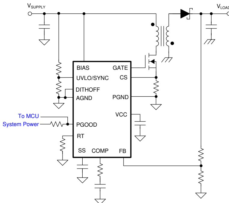
FIG 10-12. Typical Non-Isolated Flyback
