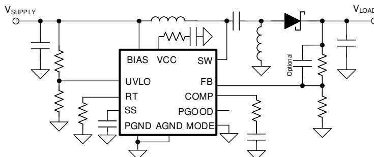
9-6. Typical SEPIC Application
