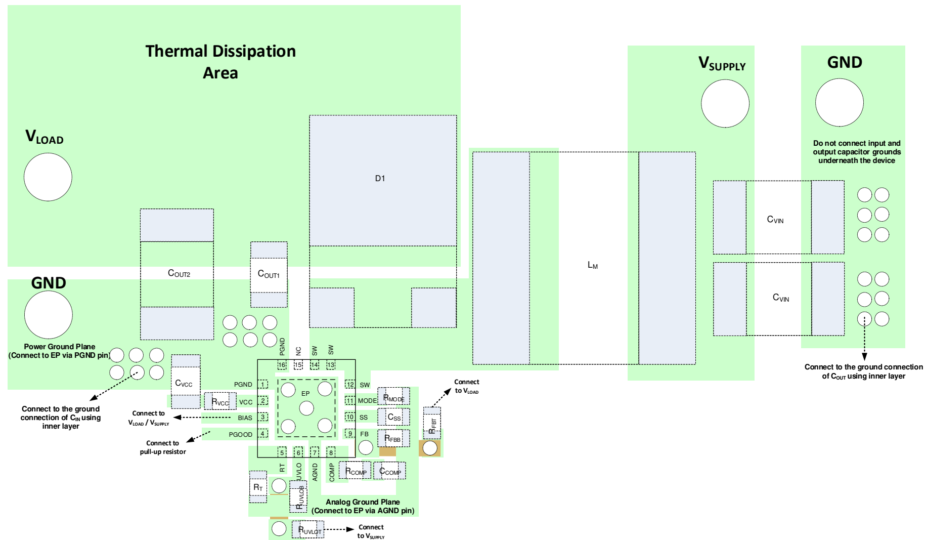
11-1. PCB Layout Example
