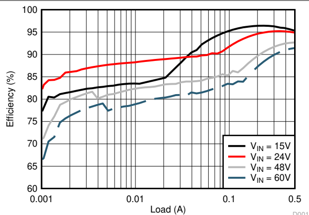
図 5-1. Conversion Efficiency (Log Scale)
