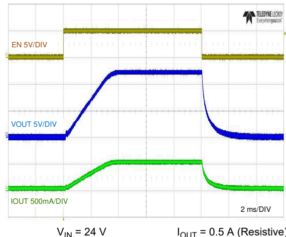
7-9. Full-Load Start-up and Shutdown with EN/UVLO
