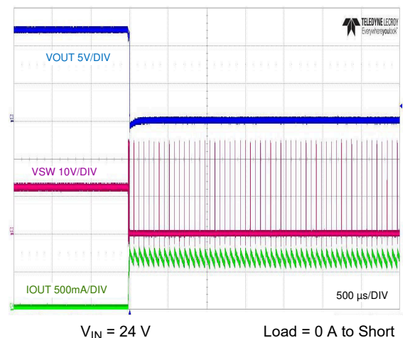
7-11. Short Circuit Applied
