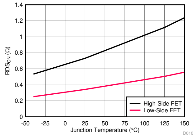
図 5-8. MOSFETs On-State Resistance versus Temperature
