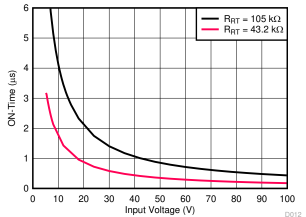
図 5-10. COT On-Time versus V_{\text{IN}}
