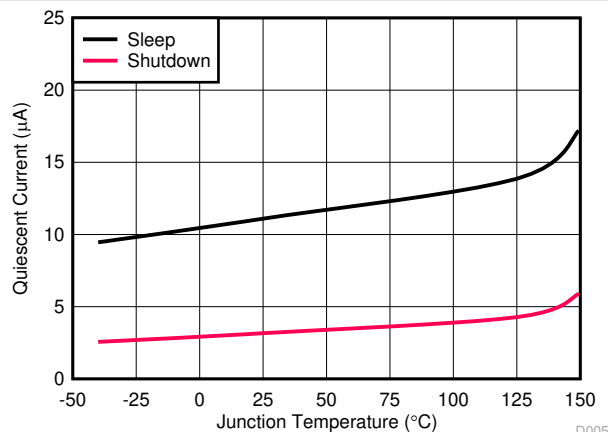
図 5-3. V_{\text{IN}} Shutdown and Sleep Supply Current versus Temperature
