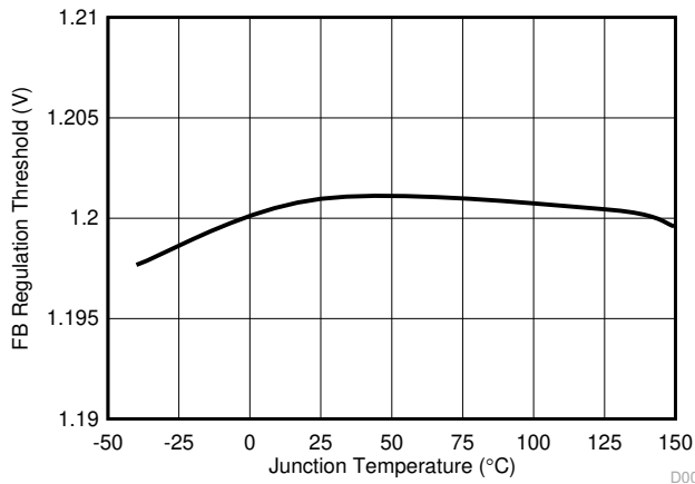
図 5-7. Feedback Comparator Threshold versus Temperature
