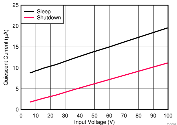
図 5-4. V_{\text{IN}} Shutdown and Sleep Supply Current versus Input Voltage
