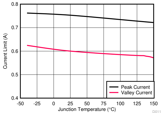
図 5-9. Peak and Valley Current Limit versus Temperature
