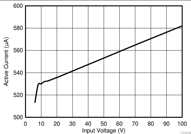
図 5-6. V_{\text{IN}} Active Current versus Input Voltage
