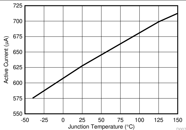
図 5-5. V_{\text{IN}} Active Current versus Temperature
