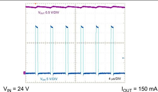
8-28. SW Node and Output Ripple Voltages, Full Load
