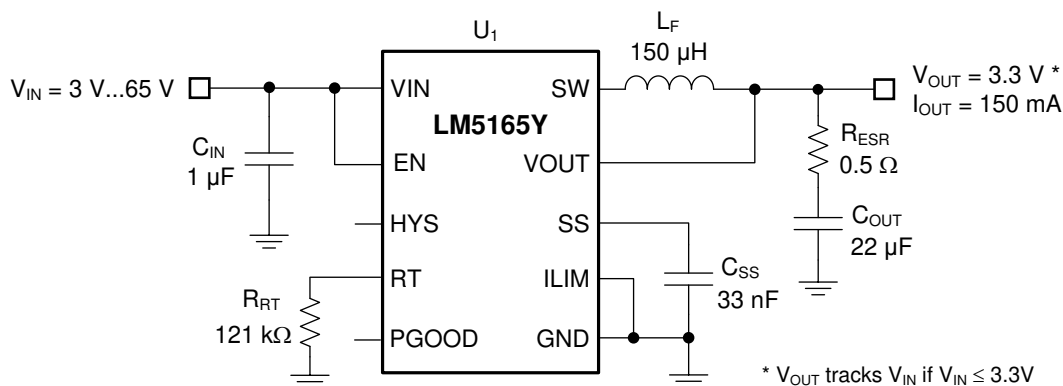
FIG 8-26. Schematic for Design 4 With V_{IN(nom)} = 24\text{ V} , V_{OUT} = 3.3\text{ V} , I_{OUT(max)} = 150\text{ mA} , F_{SW(nom)} = 160\text{ kHz}
