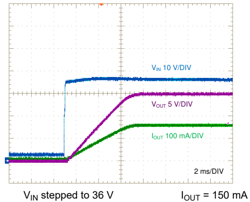
FIG 8-31. Start-Up, Full Load
