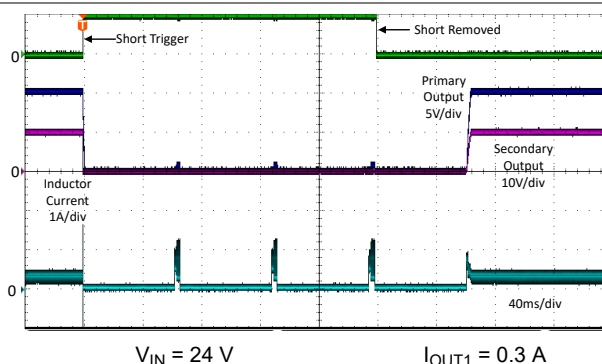
9-11. Short Circuit on Secondary Output
