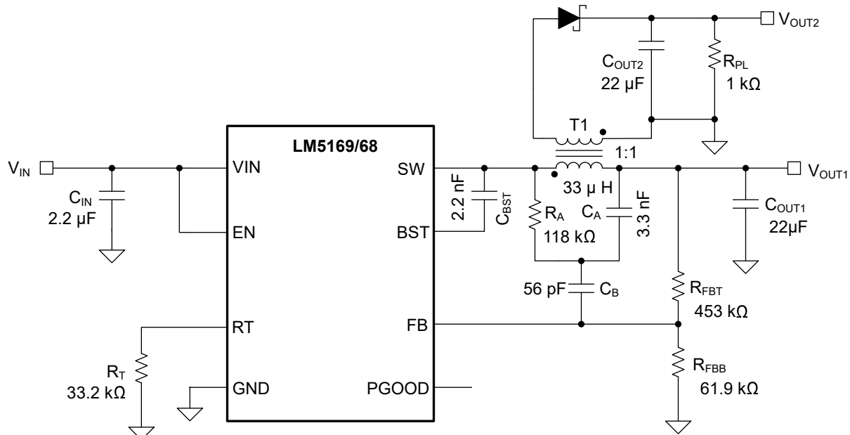
9-1. Example Fly-Buck™ Converter Application Circuit
