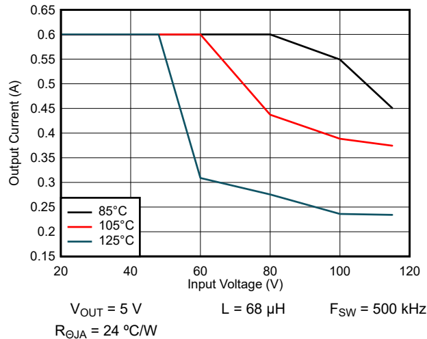
9-34. Maximum Output Current: V_{OUT} = 5\text{ V}
