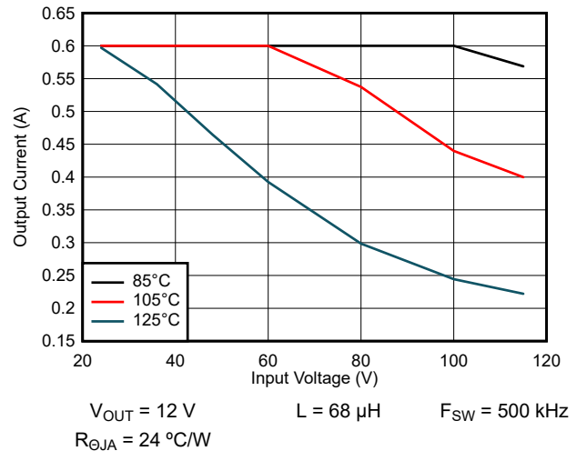
9-35. Maximum Output Current: V_{OUT} = 12\text{ V}
