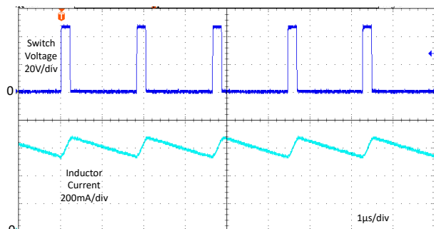
9-27. Typical Switching Waveforms
