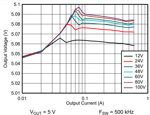
FIG 9-18. Line and Load Regulation: V_{OUT} = 5\text{ V}
