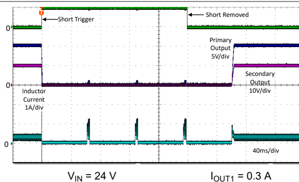
9-11. Short Circuit on Secondary Output
