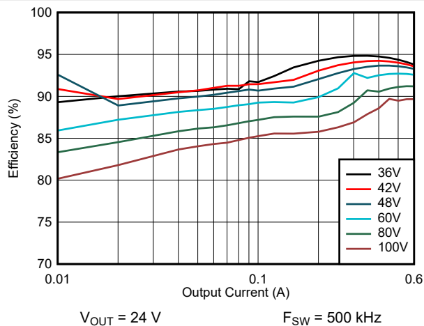
FIG 9-17. Efficiency: V_{OUT} = 24\text{ V}
