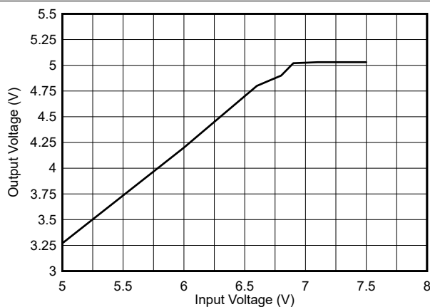
9-31. Drop-Out Response
