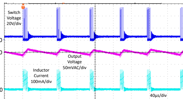
9-28. Typical Switching Waveforms
