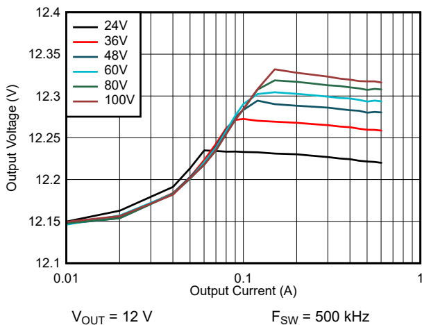
FIG 9-19. Line and Load Regulation: V_{OUT} = 12\text{ V}
