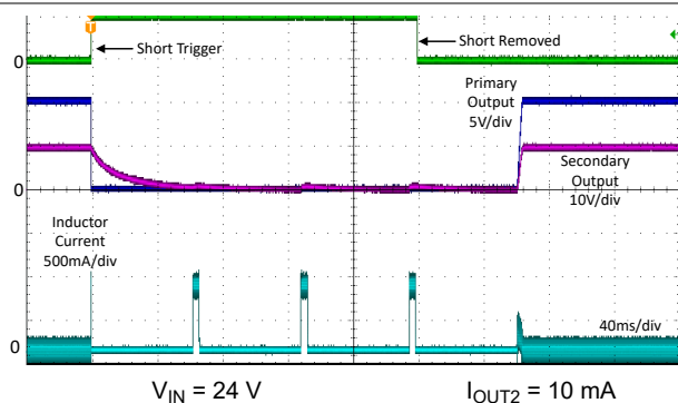
9-10. Short Circuit on Primary Output
