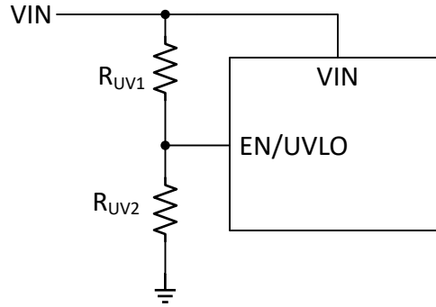
FIG 8-2. Input UVLO Connections
