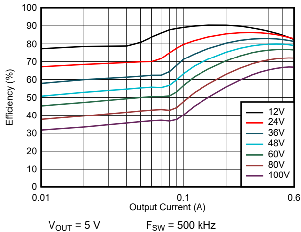
FIG 9-15. Efficiency: V_{OUT} = 5\text{ V}
