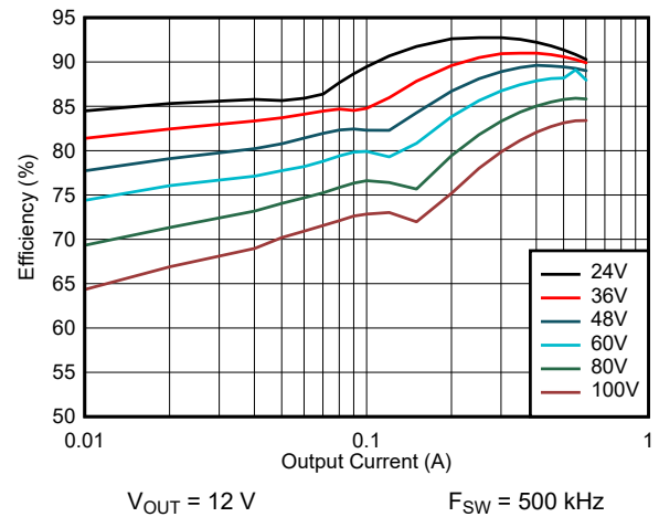
FIG 9-16. Efficiency: V_{OUT} = 12\text{ V}
