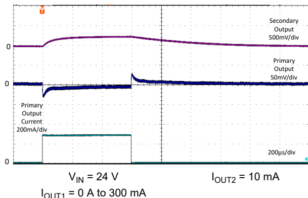
9-8. Load Transient on Primary Output
