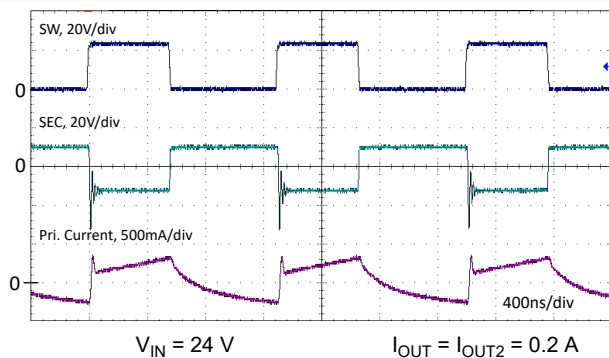
9-12. Typical Switching Waveforms
