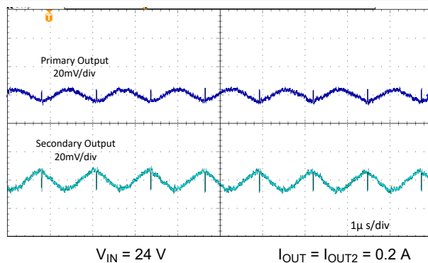
9-13. Typical Output Ripple
