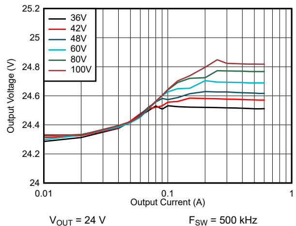
FIG 9-20. Line and Load Regulation: V_{OUT} = 24\text{ V}
