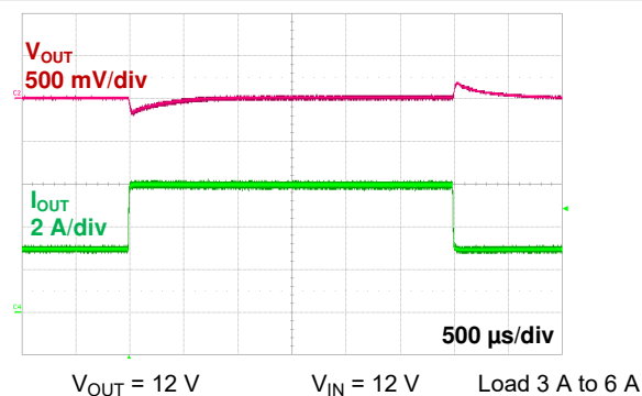
FIG 6-16. Load Step (Buck-Boost)
