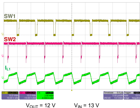
FIG 6-13. Forced CCM Operation (Buck-Boost)
