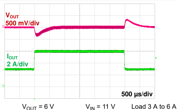
FIG 6-15. Load Step (Boost)
