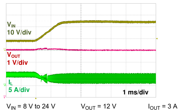
FIG 6-18. Line Transient
