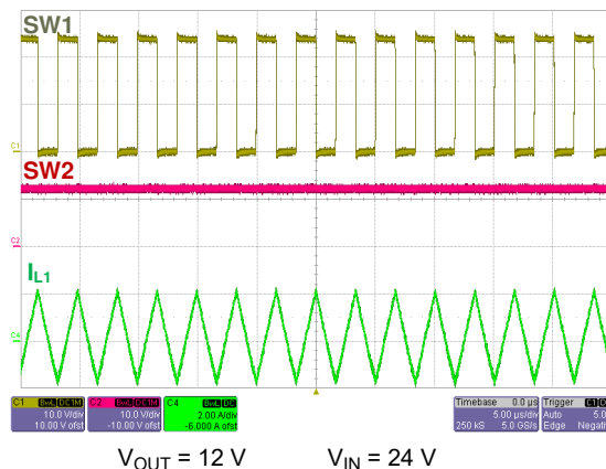
FIG 6-14. Forced CCM Operation (Buck)
