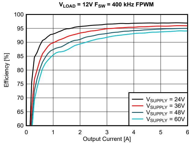
7-5. FPWM Mode Efficiency, Linear Scale
