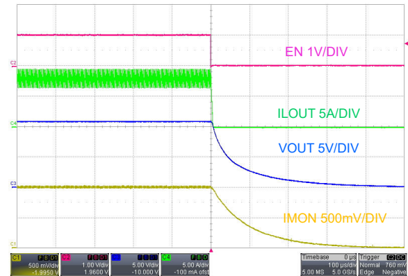
7-8. Shutdown, EN OFF, V_{SUPPLY} = 48V , I_{LOAD} = 8A Resistive Load
