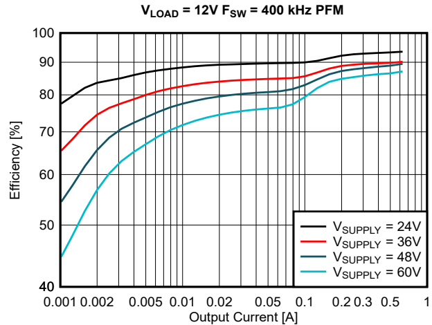
7-6. PFM Mode Efficiency, Log Scale
