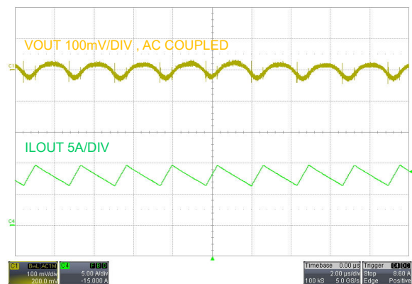
7-9. Output Ripple, V_{SUPPLY} = 48V , I_{LOAD} = 8A
