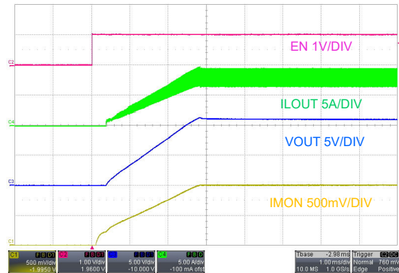
7-7. Start-Up, EN ON, V_{SUPPLY} = 48V , I_{LOAD} = 8A Resistive Load
