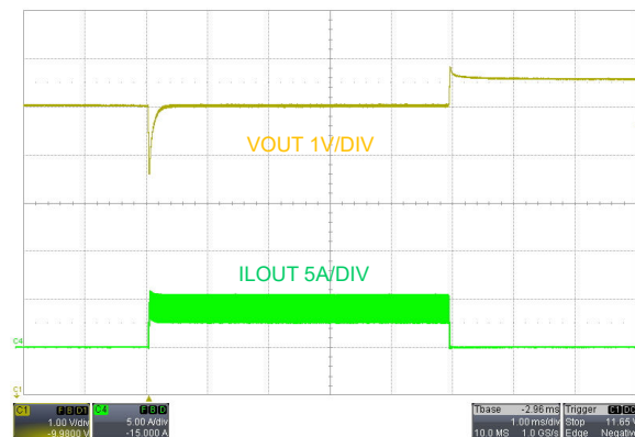
図 7-12. Load Transient Response, V_{\text{SUPPLY}} = 48\text{V} , PFM, 0A to 4A
