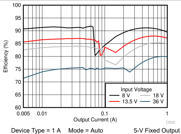
9-5. Efficiency
