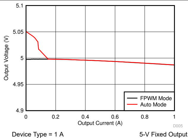
9-6. Load Regulation
