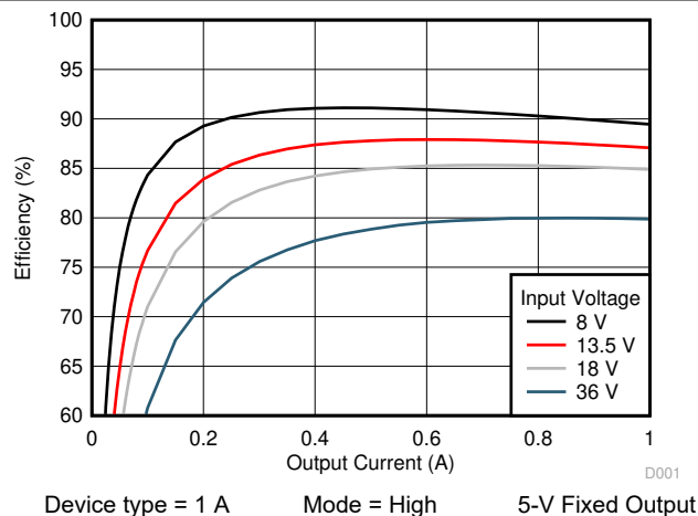
9-4. Efficiency
