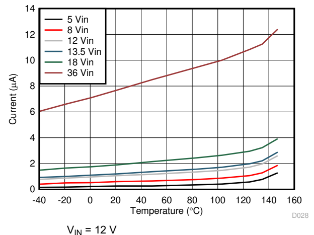
7-6. Shutdown Current
