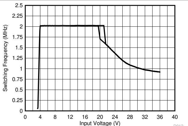
Figure 9-26. Dropout for \geq 1.85\text{ MHz}
