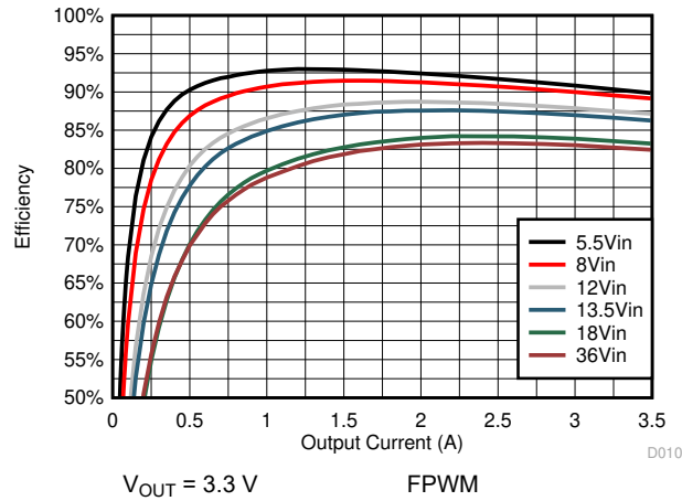
9-21. Efficiency
