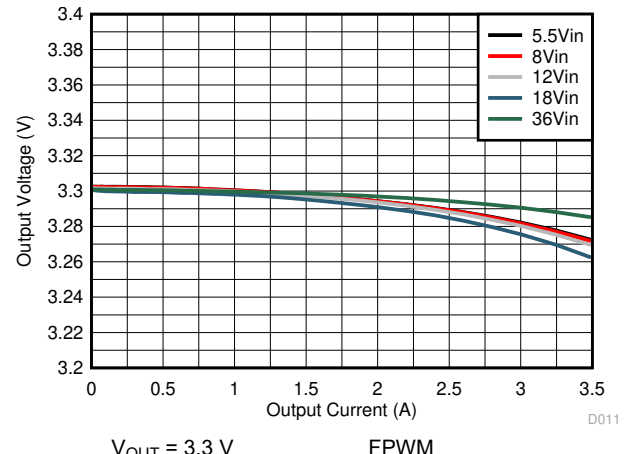
9-22. Load and Line Regulation
