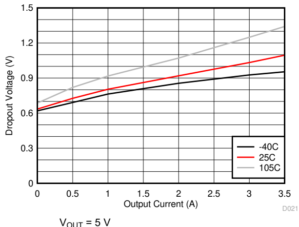
Figure 9-12. Dropout for \geq 1.85 MHz
