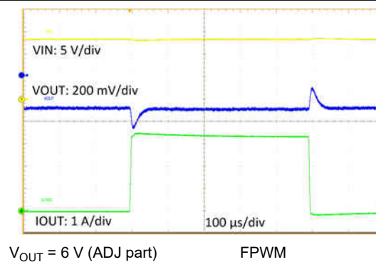
Figure 9-38. Load Transient
