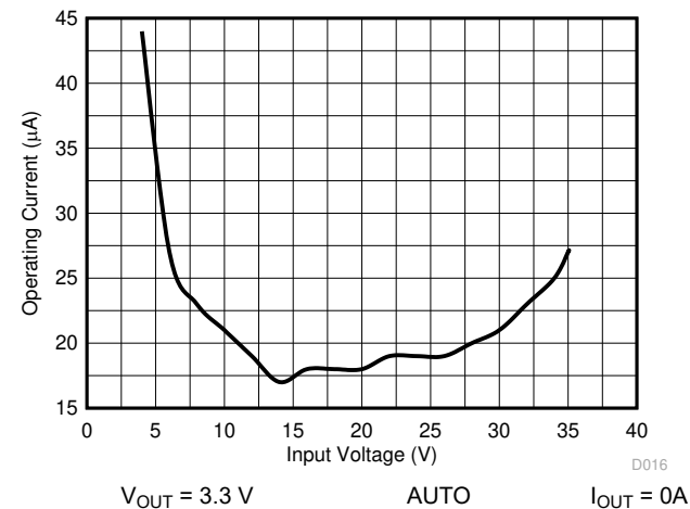
9-23. Input Supply Current (Includes Leakage Current of Capacitor)
