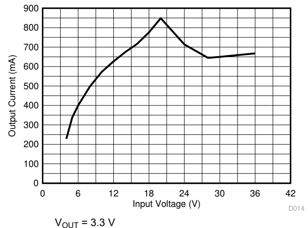
9-24. Load Current for PFM-to-PWM Transition
