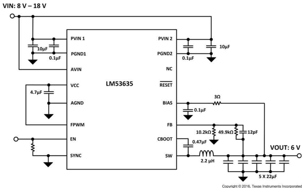
✎ 9-34. 6 V Output Power Supply
