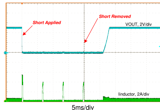
図 8-6. Short-Circuit Transient and Recovery
