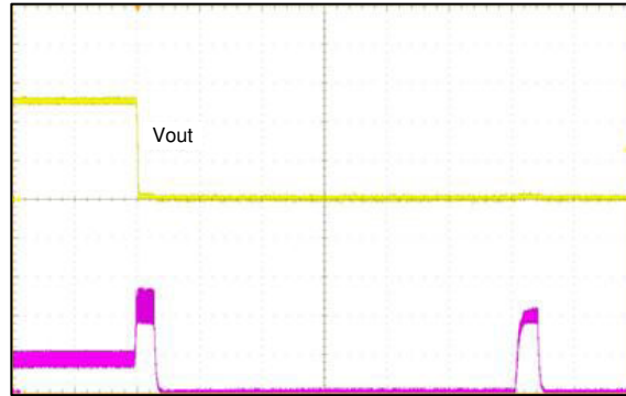
8-7. Hiccup Operation
