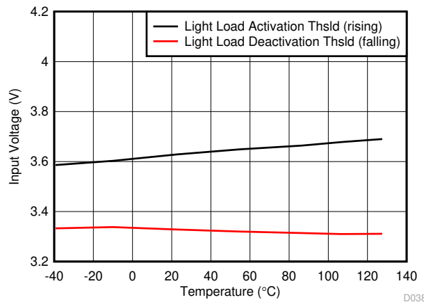
Figure 8-10. Input Voltage for Mode Change — Fixed 3.3-V Output, 2.2-μH Inductor
