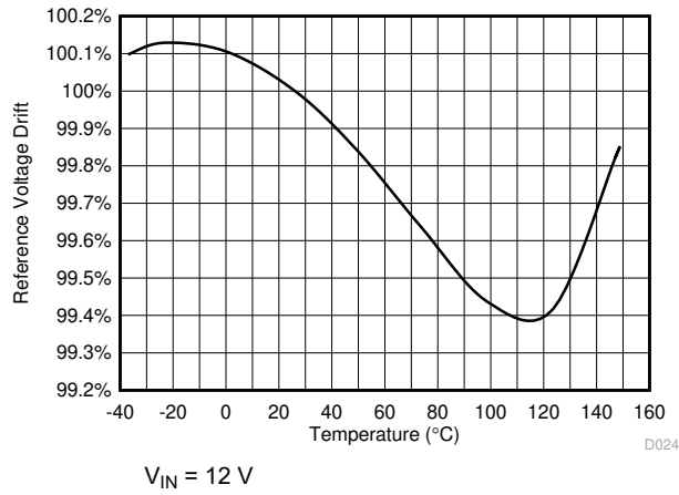
7-1. Reference Voltage Drift
