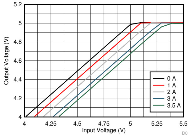
FIG 8-11. Overall Dropout Characteristics ( V_{OUT} = 5 V)
