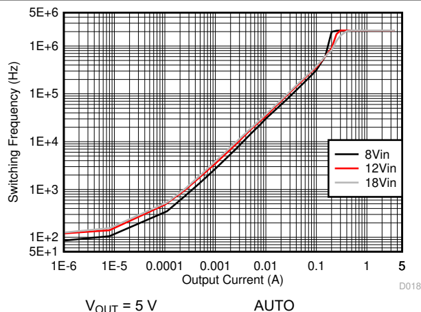
Figure 9-13. Switching Frequency vs Load Current
