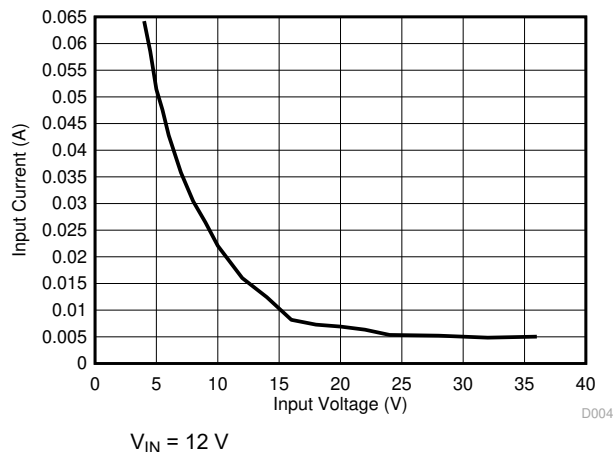
7-5. Short Circuit Average Input Current for LM53635-Q1
