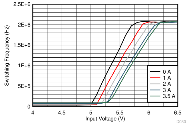
FIG 8-12. Frequency Dropout Characteristics ( V_{OUT} = 5 V)
