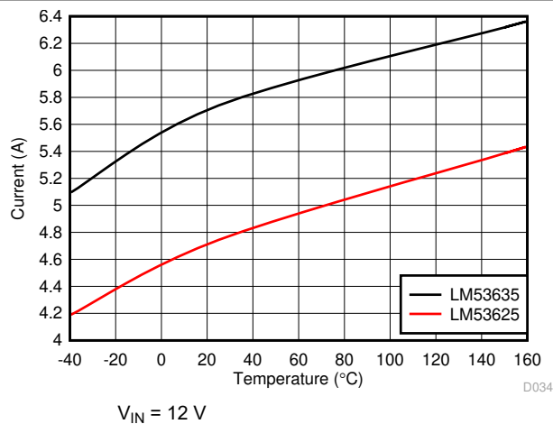
7-3. High Side/Peak Current Limit for LM53625/35-Q1
