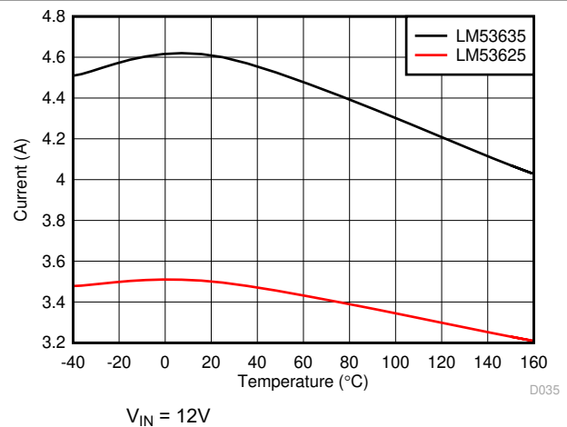
7-4. Low Side/Valley Current Limit for LM53625/35-Q1
