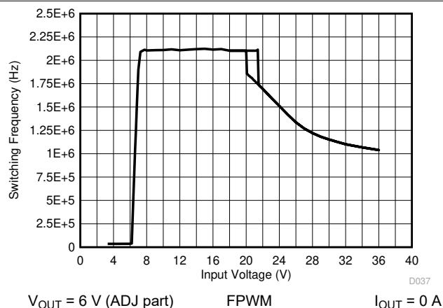
Figure 9-35. Switching Frequency vs Input Voltage
