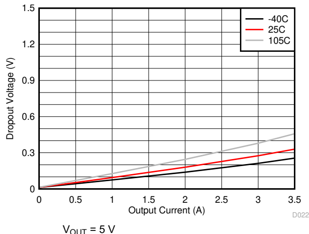
Figure 9-11. Dropout for -3% Regulation
