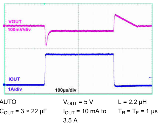
Figure 9-16. Load Transients
