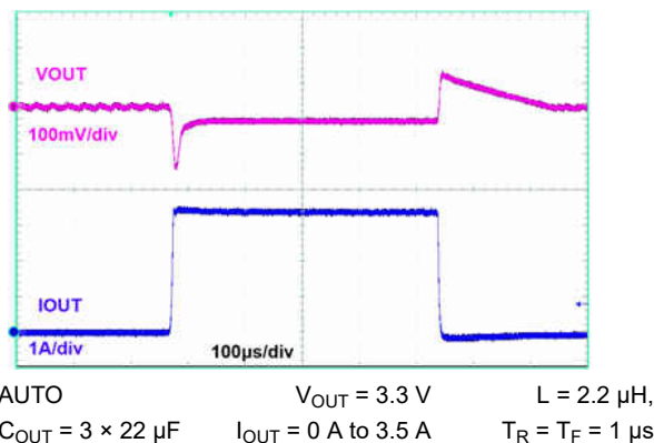
Figure 9-30. Load Transient
