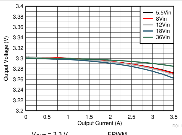
9-22. Load and Line Regulation
