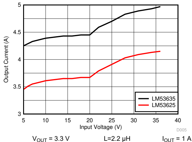
Figure 9-29. Output Current Level for Overcurrent Protection Trip
