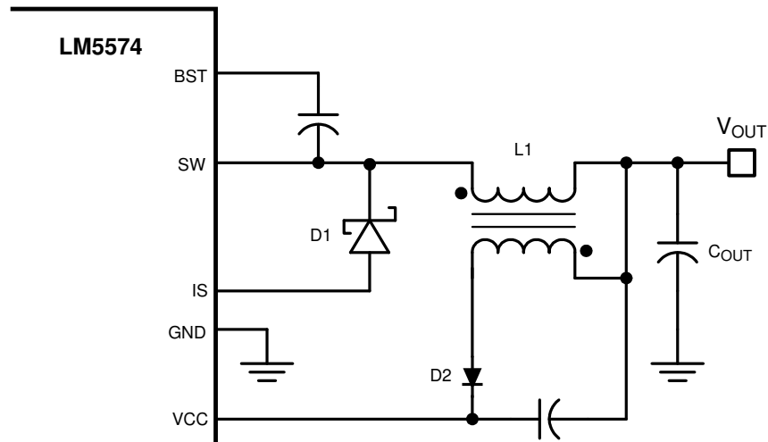
図 7-2. VCC Bias With Additional Winding on the Output Inductor
