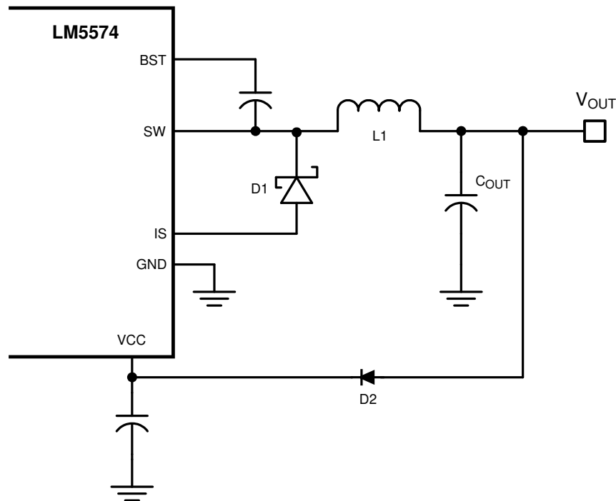
図 7-1. VCC Bias From VOUT for 8V < V_{OUT} < 14V
