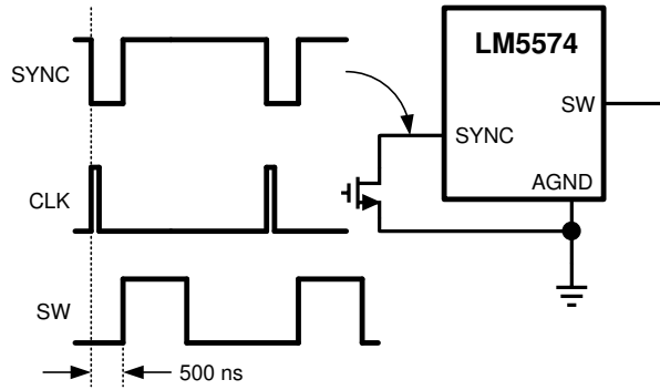
図 6-2. Sync From External Clock
