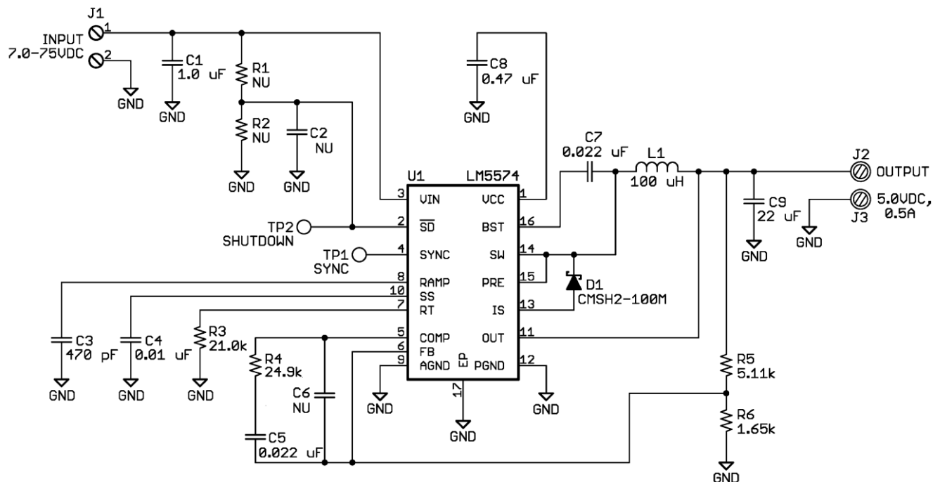
図 7-3. Typical Application Schematic
