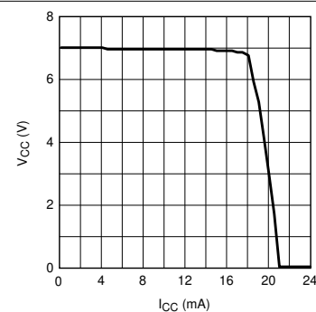
Figure 5-4. V_{CC} vs I_{CC} V_{IN} = 12\text{V}
