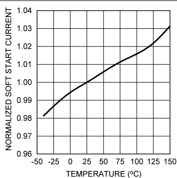
Figure 5-3. Soft-Start Current vs Temperature
