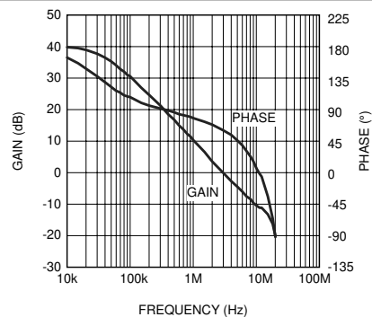
Figure 5-6. Error Amplifier Gain And Phase A_{VCL} = 101
