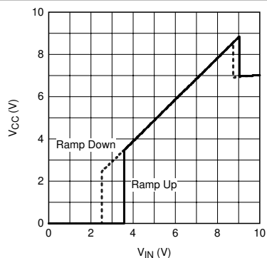
Figure 5-5. V_{CC} vs V_{IN} R_L = 7\text{k}\Omega
