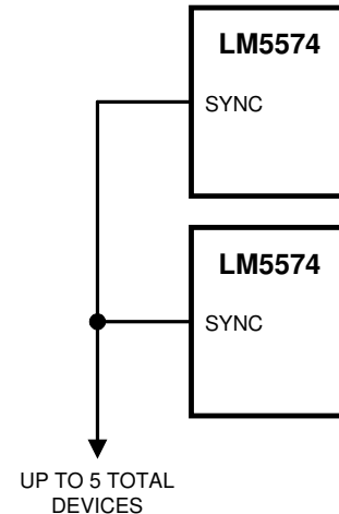
図 6-3. Sync From Multiple Devices
