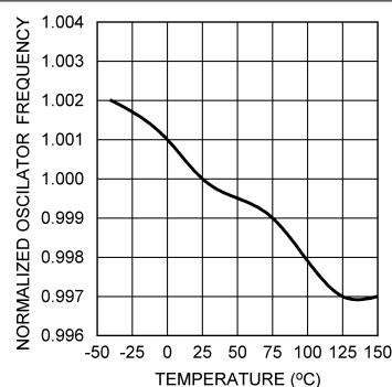
Figure 5-2. Oscillator Frequency vs Temperature F_{OSC} = 200\text{kHz}
