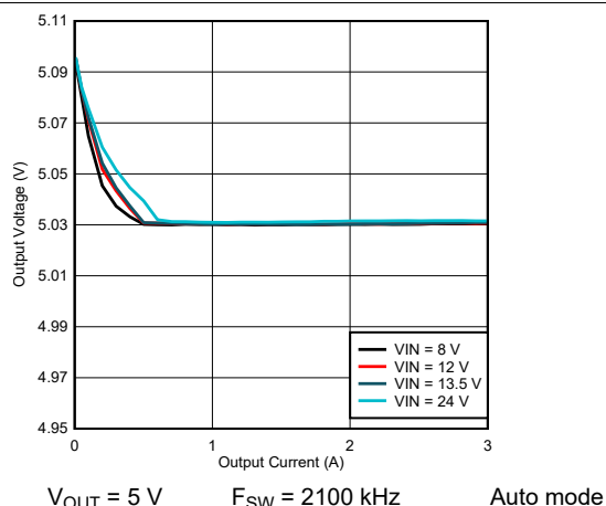
Figure 9-18. LM61430-Q1 Load and Line Regulation
