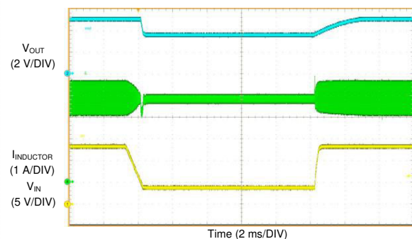
9-43. LM61460 Short Circuit Recovery
