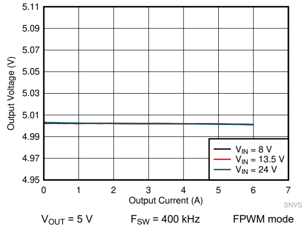
9-24. LM61460 Load and Line Regulation
