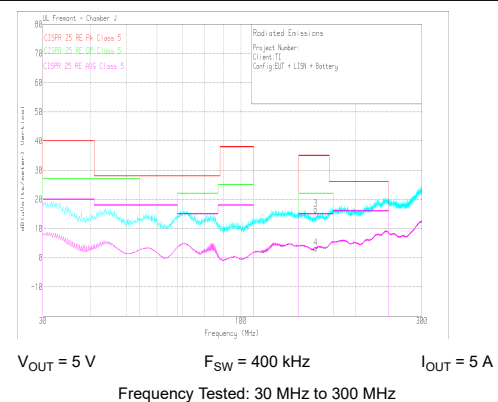
9-58. Radiated EMI Bicon Horizontal versus CISPR25 Limits
