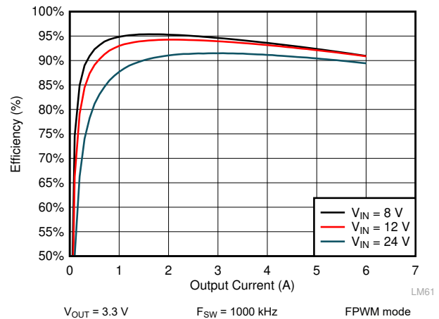
Figure 9-8. LM61460 Efficiency
