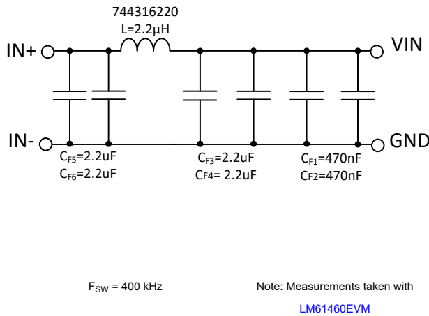
9-61. Recommended Input EMI Filter
