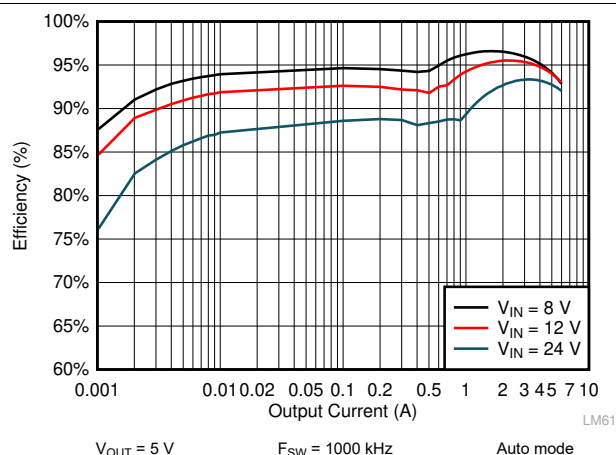
9-13. LM61460 Efficiency
