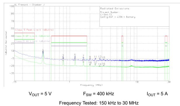
9-56. Radiated EMI Rod versus CISPR25 Limits
