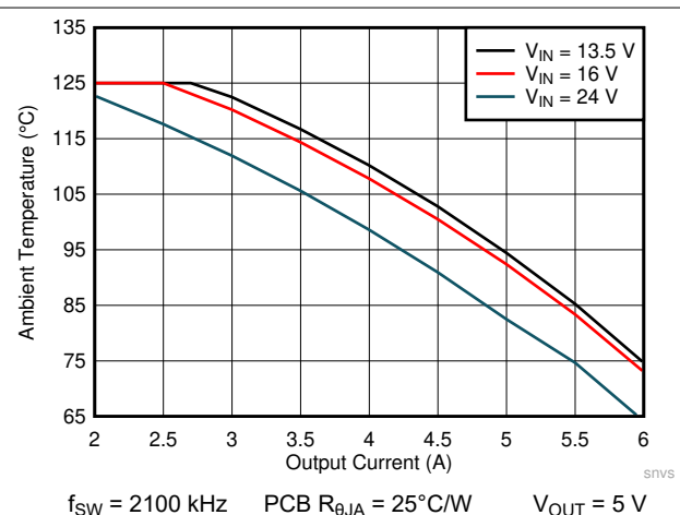
図 9-3. Maximum Ambient Temperature Versus Output Current
