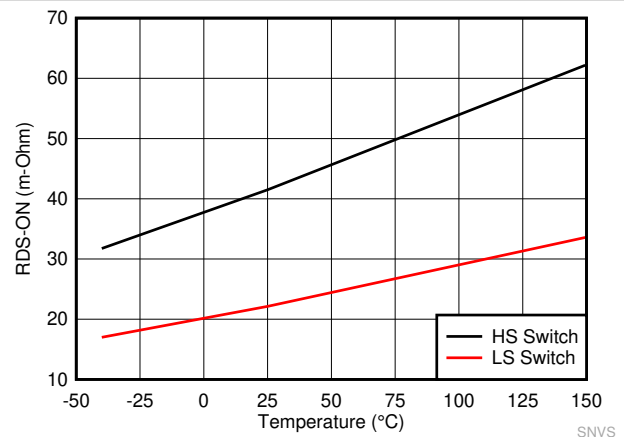
7-6. High-Side and Low-Side Switches R_{DS-ON}
