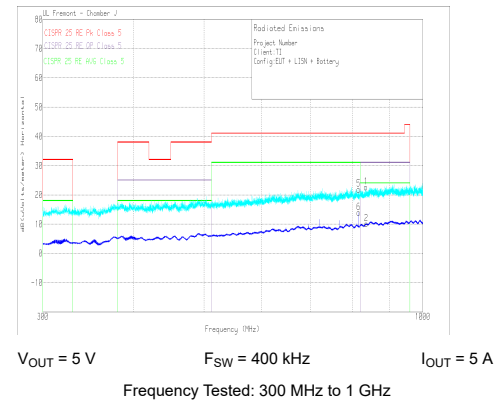
9-60. Radiated EMI Log Horizontal versus CISPR25 Limits
