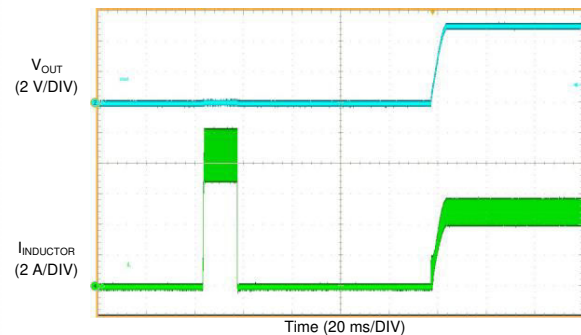
9-41. LM61460 Start-up with 3.25-A
