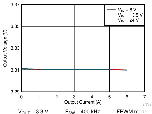
9-18. LM61460 Load and Line Regulation
