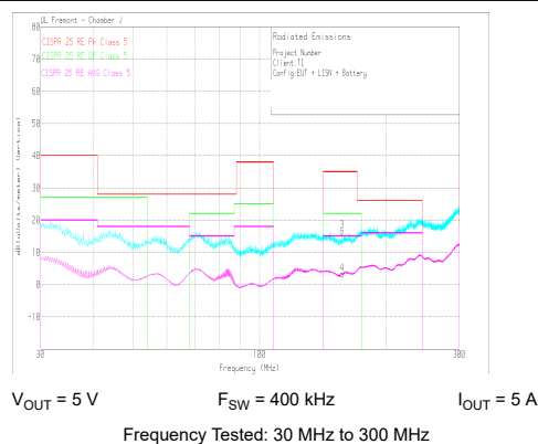
9-57. Radiated EMI Bicon Vertical versus CISPR25 Limits
