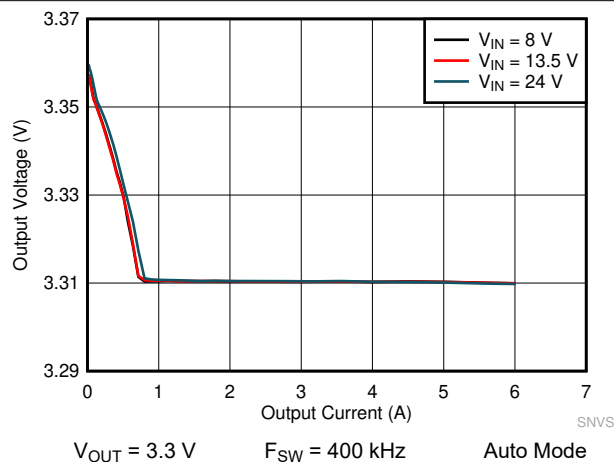
9-17. LM61460 Load and Line Regulation
