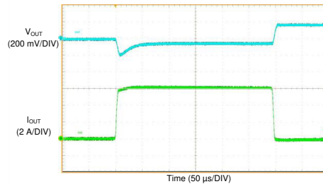
9-48. LM61460 Load Transient
