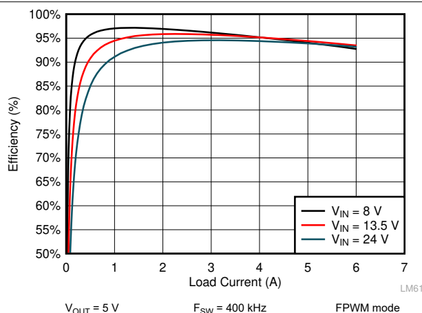
9-12. LM61460 Efficiency
