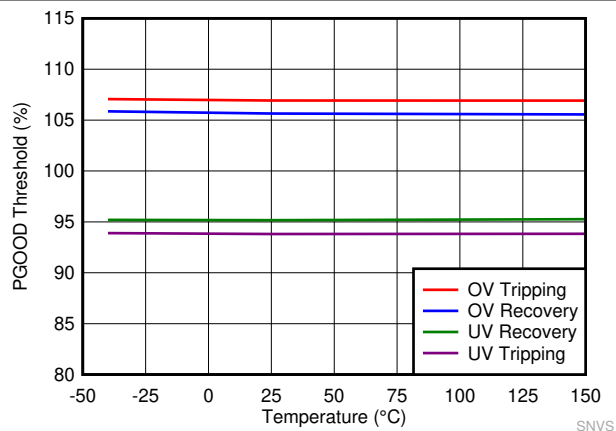
7-8. PGOOD Thresholds
