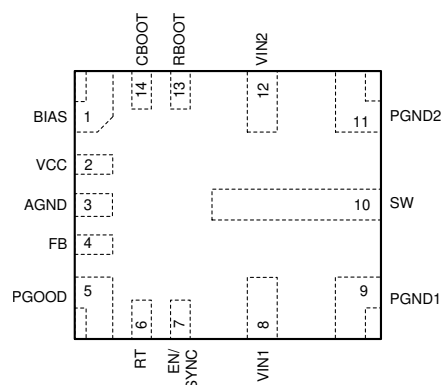
図 6-1. 14-Pin VQFN-HR RJR Package (Top View)
