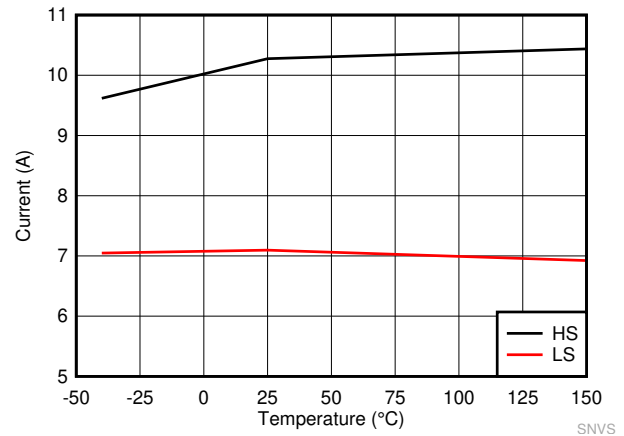
7-4. LM61460 High-Side and Low-Side Current Limits
