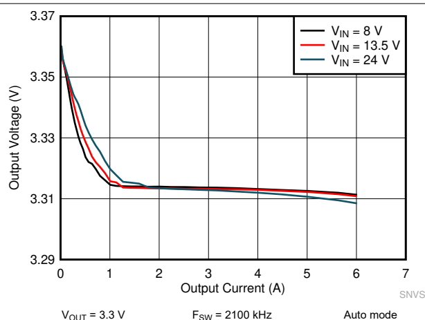
9-21. LM61460 Load and Line Regulation
