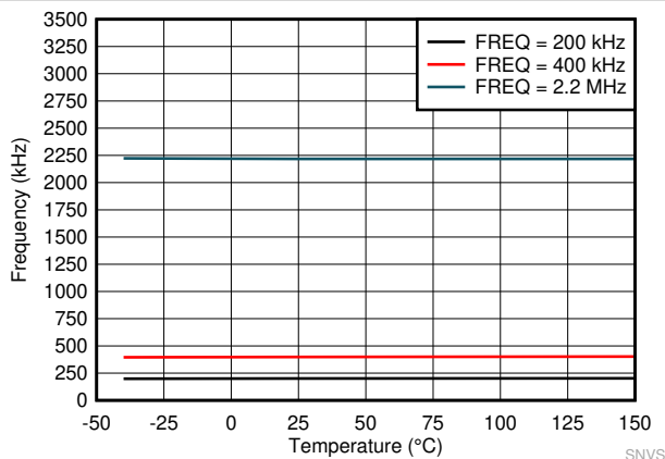
7-5. Switching Frequency Set by RT Resistor
