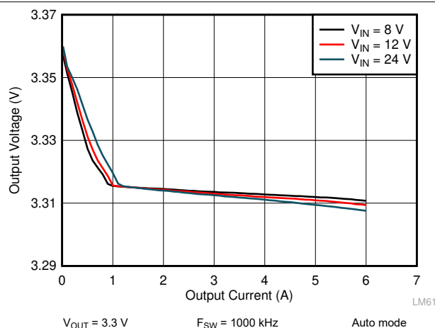
9-19. LM61460 Load and Line Regulation
