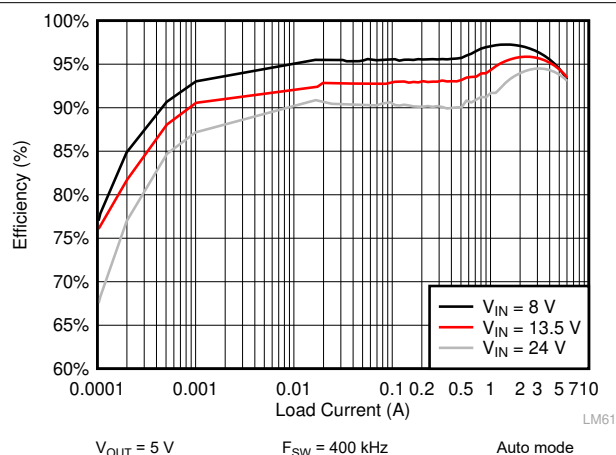
9-11. LM61460 Efficiency
