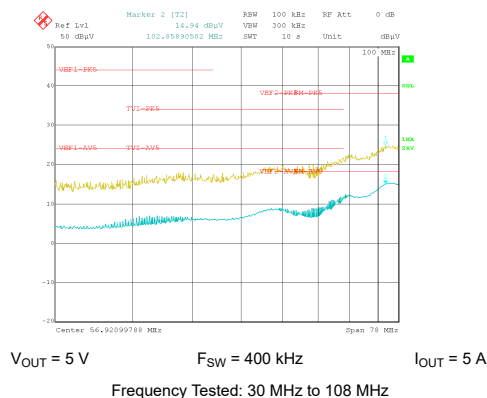
9-55. Conducted EMI versus CISPR25 Limits (Yellow: Peak Signal, Blue: Average Signal)
