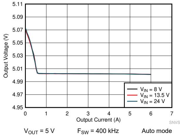
9-23. LM61460 Load and Line Regulation
