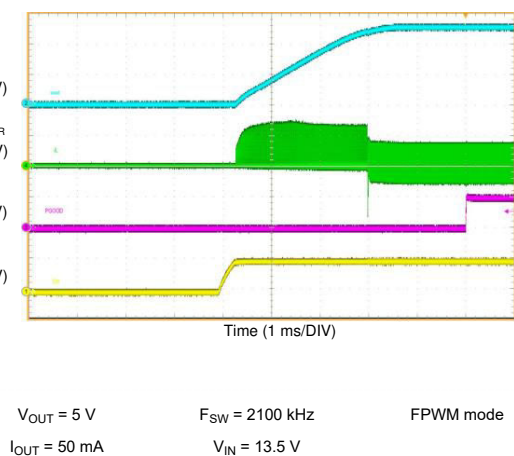
Figure 9-40. LM61460 Start-up with 50-mA
