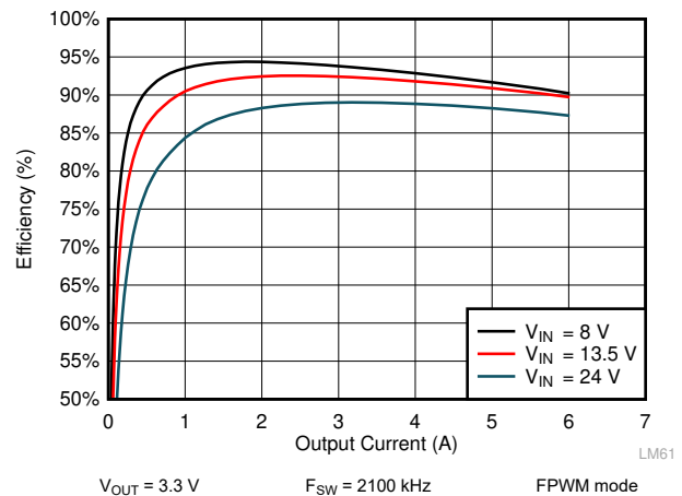
Figure 9-10. LM61460 Efficiency
