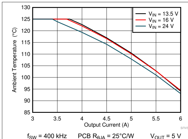
図 9-2. Maximum Ambient Temperature Versus Output Current
