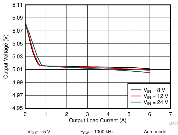
9-25. LM61460 Load and Line Regulation
