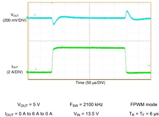
9-53. LM61460 Load Transient
