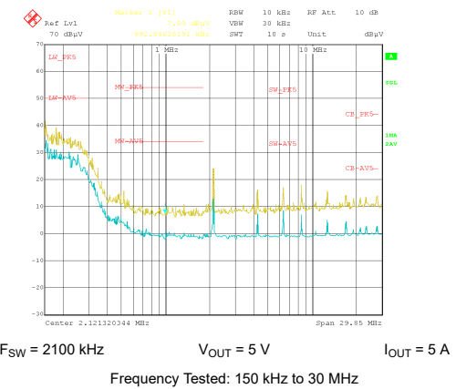
9-62. Conducted EMI versus CISPR25 Limits (Yellow: Peak Signal, Blue: Average Signal)
