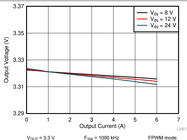
9-20. LM61460 Load and Line Regulation
