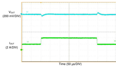
9-49. LM61460 Load Transient
