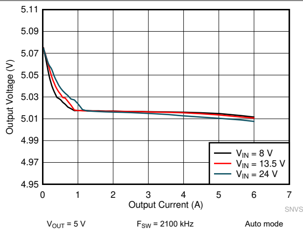
9-27. LM61460 Load and Line Regulation
