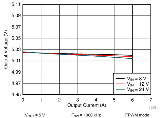
9-26. LM61460 Load and Line Regulation
