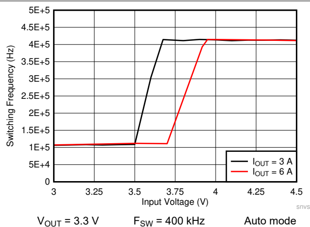
9-33. LM61460 Frequency Dropout Curve
