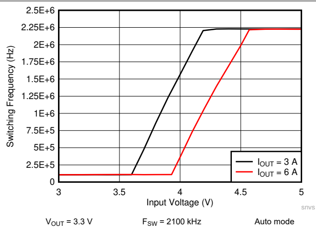
9-34. LM61460 Frequency Dropout Curve
