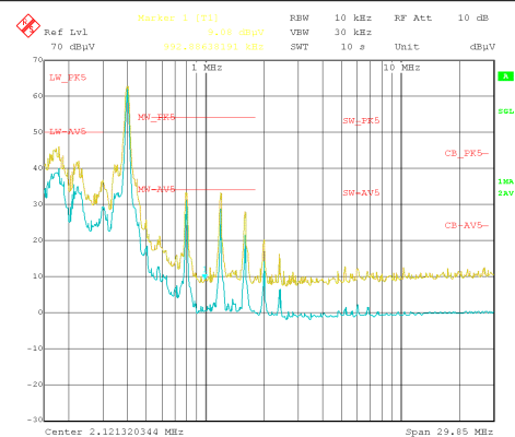
9-54. Conducted EMI versus CISPR25 Limits (Yellow: Peak Signal, Blue: Average Signal)
