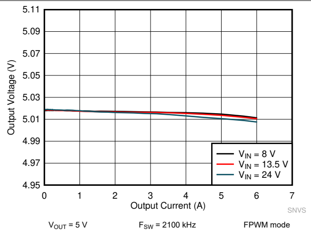
9-28. LM61460 Load and Line Regulation
