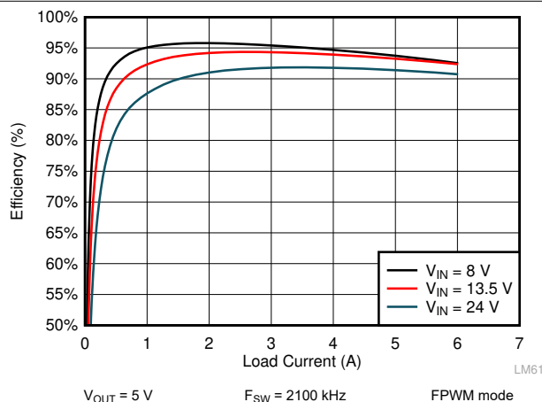
9-16. LM61460 Efficiency
