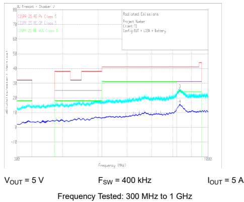
9-59. Radiated EMI Log Vertical versus CISPR25 Limits
