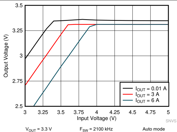
9-30. LM61460 Dropout Curve
