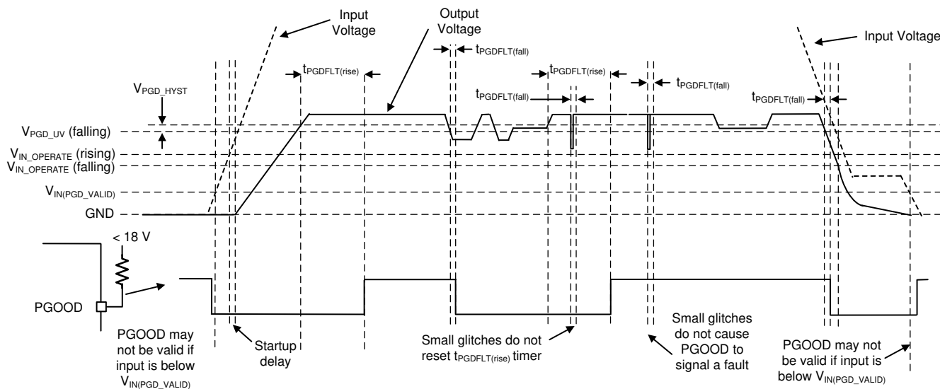
8-6. PGOOD Timing Diagram (Excludes OV Events)
