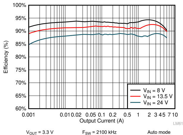
Figure 9-9. LM61460 Efficiency
