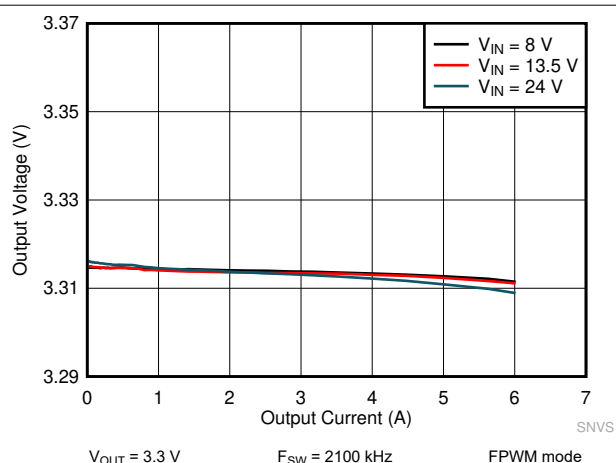
9-22. LM61460 Load and Line Regulation
