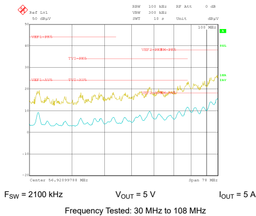
9-63. Conducted EMI versus CISPR25 Limits (Yellow: Peak Signal, Blue: Average Signal)
