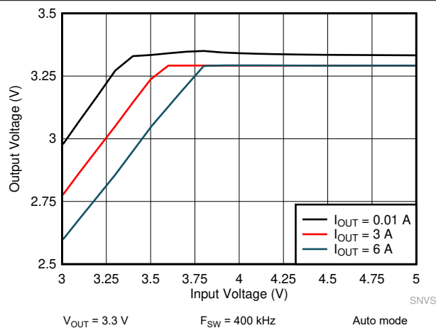
9-29. LM61460 Dropout Curve
