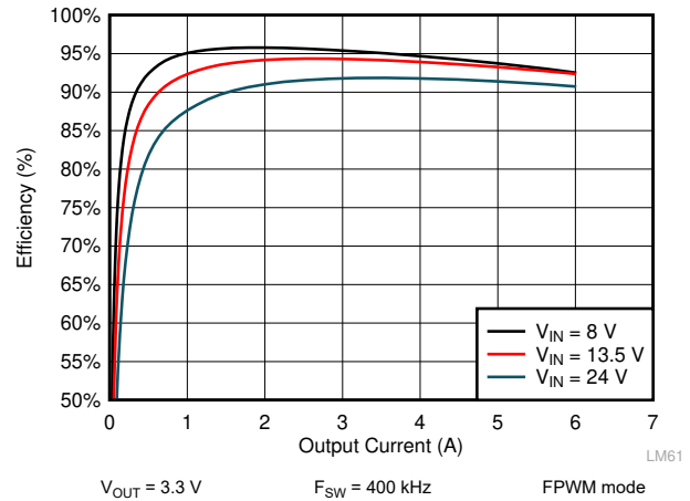
Figure 9-6. LM61460 Efficiency
