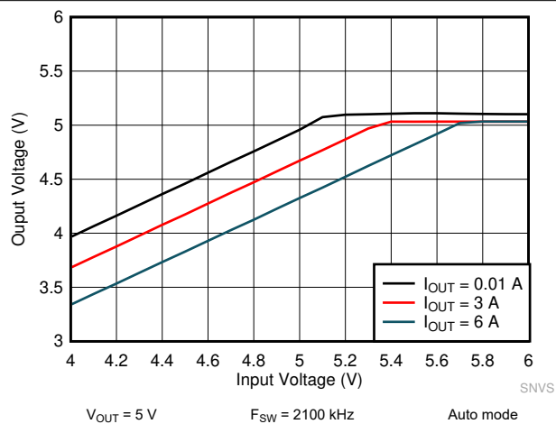
9-32. LM61460 Dropout Curve
