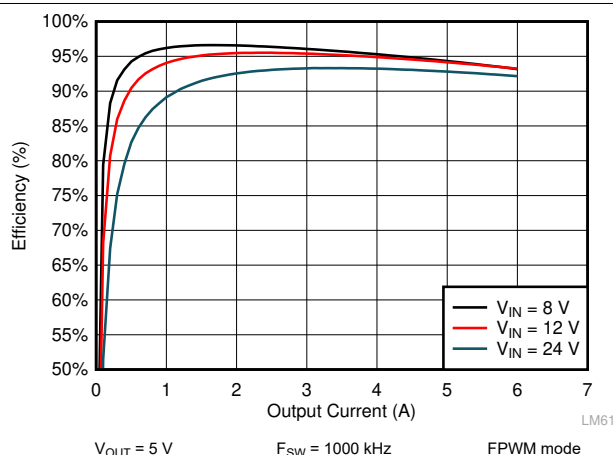
9-14. LM61460 Efficiency
