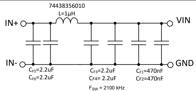
9-64. Recommended Input EMI Filter
