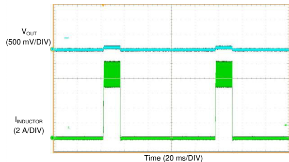
9-42. LM61460 Short Circuit Protection
