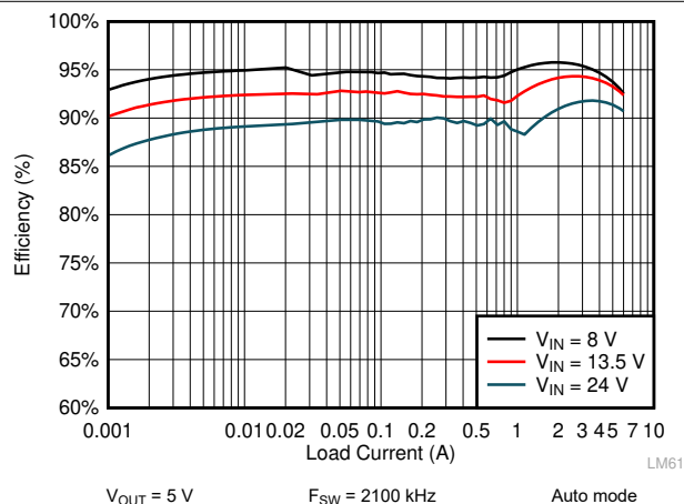
9-15. LM61460 Efficiency
