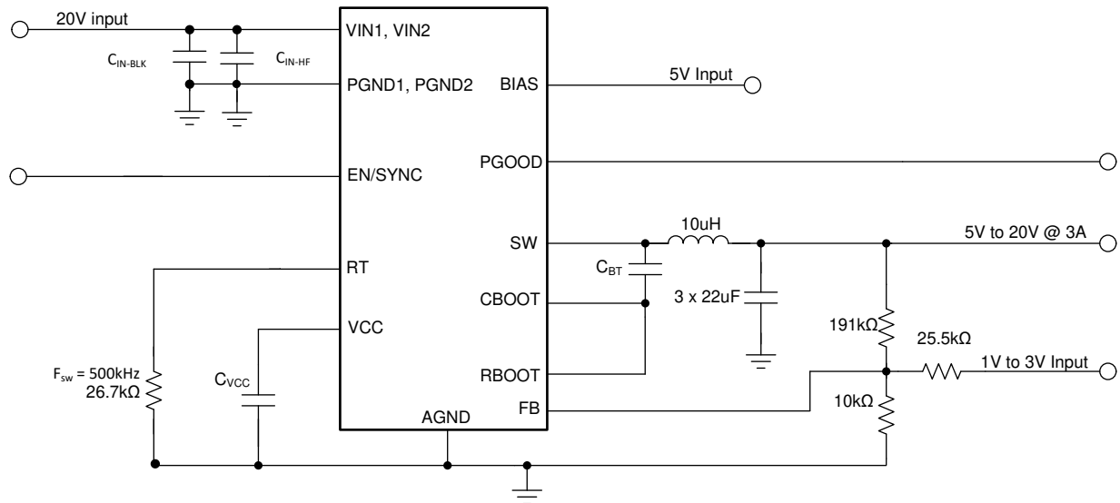
図 9-65. USB Type-C Power Supply
