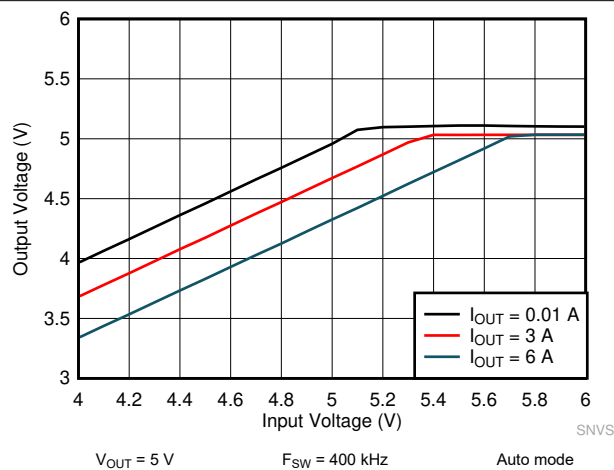
9-31. Dropout Curve
