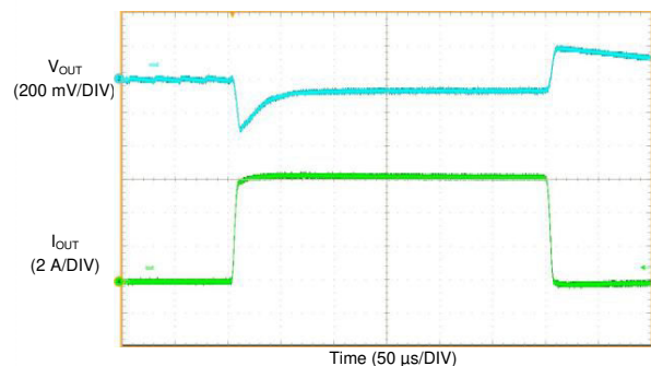
9-47. LM61460 Load Transient
