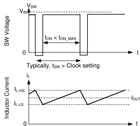
8-18. Current Limit Waveforms
