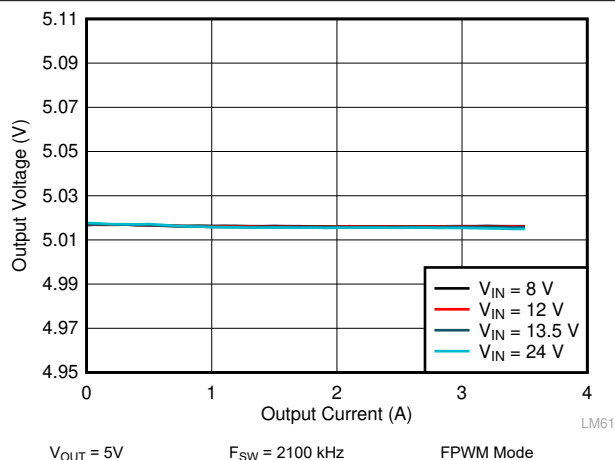
图 9-12. LM62435-Q1 Load and Line Regulation
