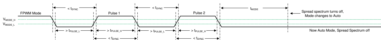
图 8-8. Spread Spectrum Disabled in Transition from FPWM Mode to Auto Mode
