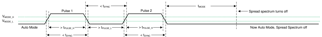
图 8-7. Spread Spectrum Disabled in Auto Mode
