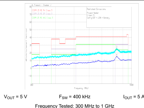
FIG 9-30. Radiated EMI Log Vertical versus CISPR25 Limits
