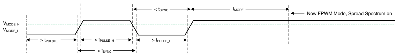
图 8-11. Transition from SYNC Mode to FPWM Mode
