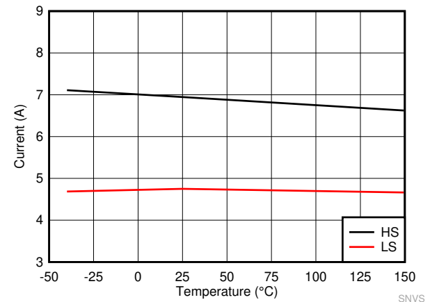
图 7-4. LM62435-Q1 High-side and Low-side Current Limits
