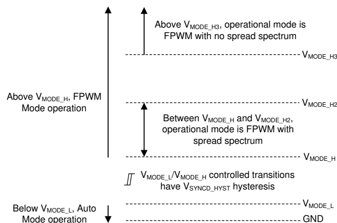
図 8-2. Level-Dependent Mode Selection Settings
