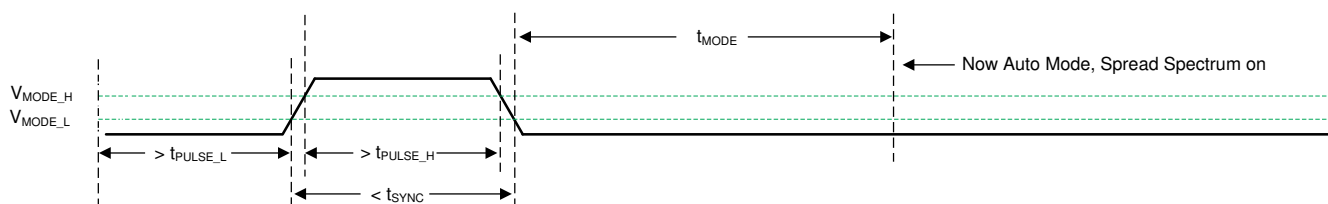
图 8-10. Transition from SYNC Mode to Auto Mode
