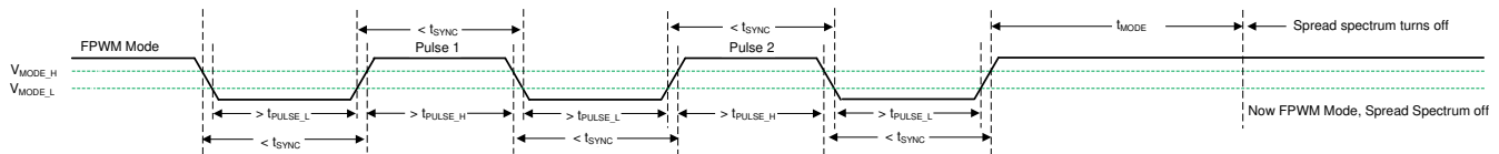
图 8-6. Spread Spectrum Disabled in FPWM Mode
