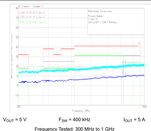
FIG 9-31. Radiated EMI Log Horizontal versus CISPR25 Limits
