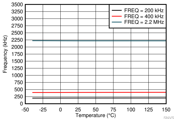
图 7-5. Switching Frequency Set by SYNC
