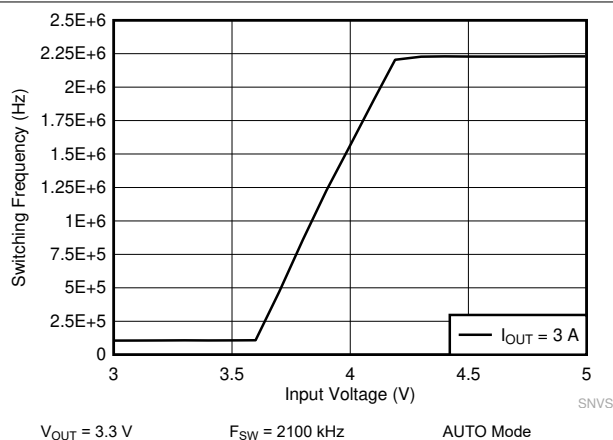
图 9-15. LM62435-Q1 Frequency Dropout Curve
