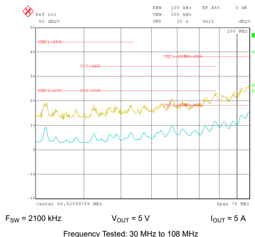
FIG 9-34. Conducted EMI versus CISPR25 Limits (Yellow: Peak Signal, Blue: Average Signal)
