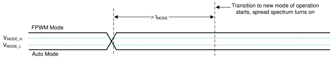
图 8-5. Transition from Auto Mode and FPWM Mode
