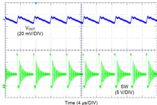
图 9-17. LM62435-Q1 Switching Waveform and V_{OUT} Ripple
