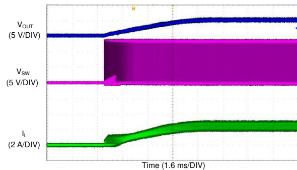
Figure 8-20. Short Circuit Recovery
