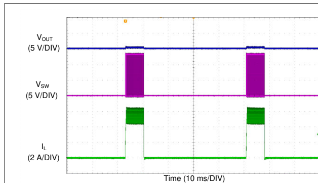
Figure 8-19. Inductor Current Bursts During Hiccup
