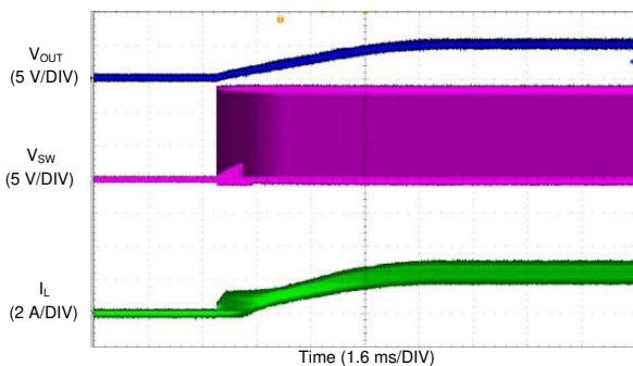
图 9-19. LM62435-Q1 Start-up with 3.25 A
