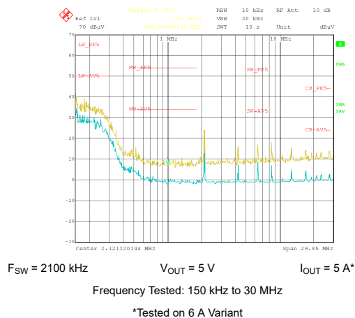
FIG 9-33. Conducted EMI versus CISPR25 Limits (Yellow: Peak Signal, Blue: Average Signal)
