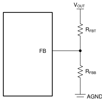
FIG 8-17. Setting Output Voltage of Adjustable Versions
