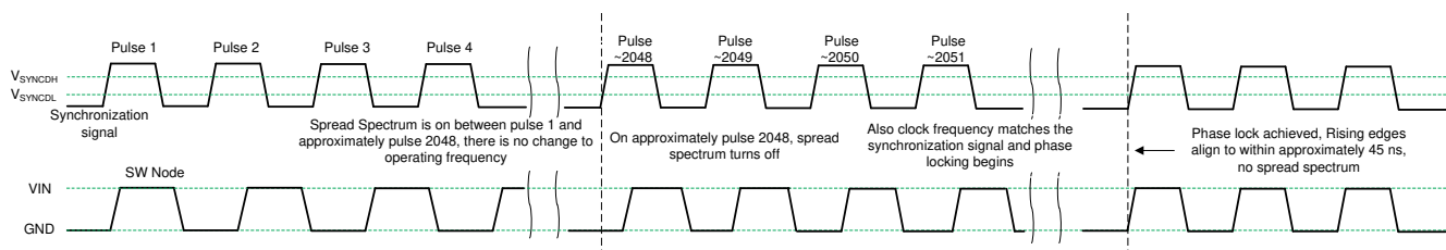
图 8-12. Synchronization Process
