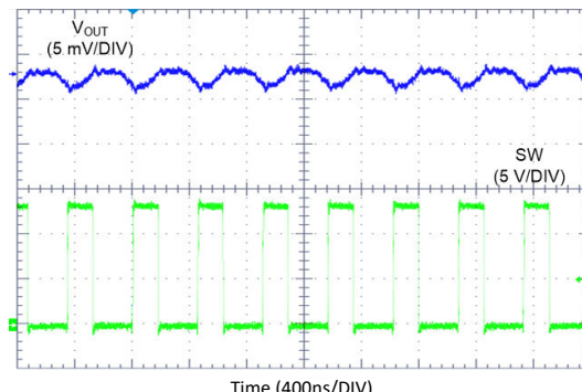
图 9-18. LM62435-Q1 Switching Waveform and V_{OUT} Ripple
