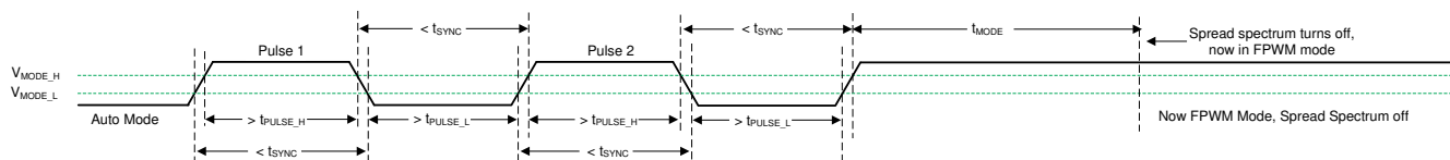
图 8-9. Spread Spectrum Disabled in Transition from Auto Mode to FPWM Mode
