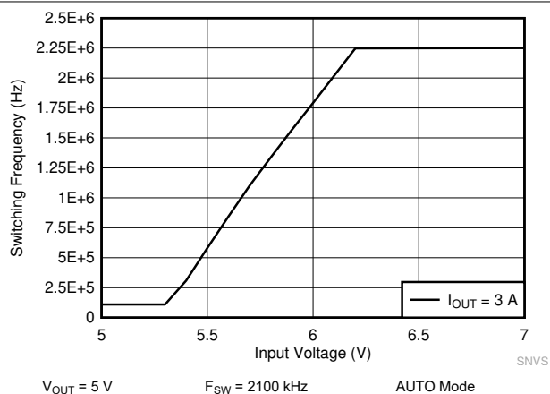
图 9-16. LM62435-Q1 Frequency Dropout Curve
