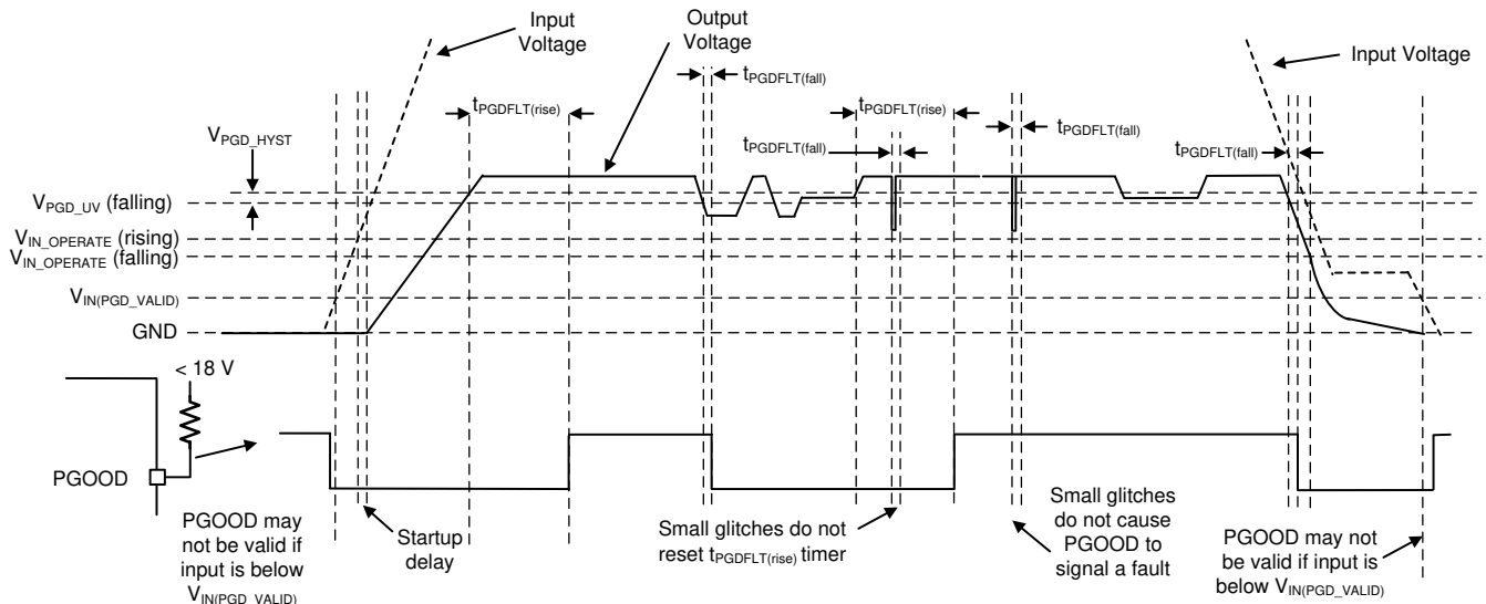
図 8-13. PGOOD Timing Diagram (Excludes OV Events)
