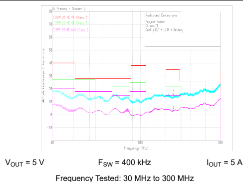
FIG 9-29. Radiated EMI Bicon Horizontal versus CISPR25 Limits
