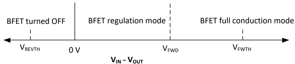
7-6. Reverse Current Blocking Response
