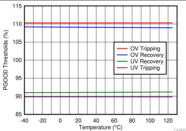
7-9. PGOOD Thresholds
