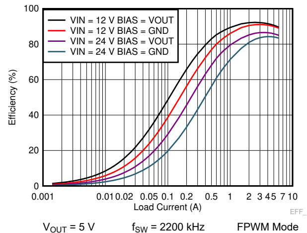
☒ 8-7. LM73606-Q1 Efficiency Comparison With Bias = V_{\text{OUT}} to Bias = GND in FPWM Mode
