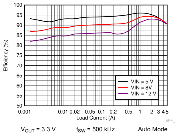
9-5. LM73605-Q1 Efficiency
