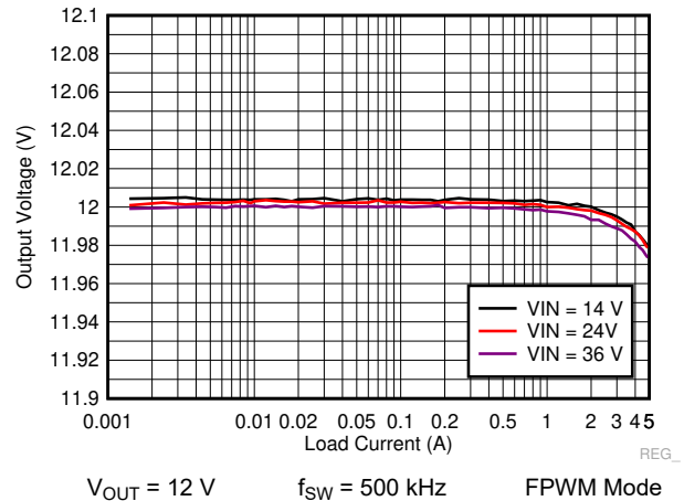
FIG 9-34. LM73605-Q1 Load and Line Regulation
