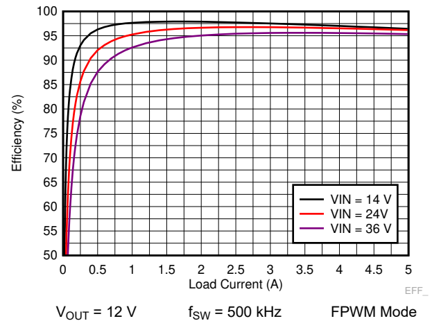
9-20. LM73605-Q1 Efficiency
