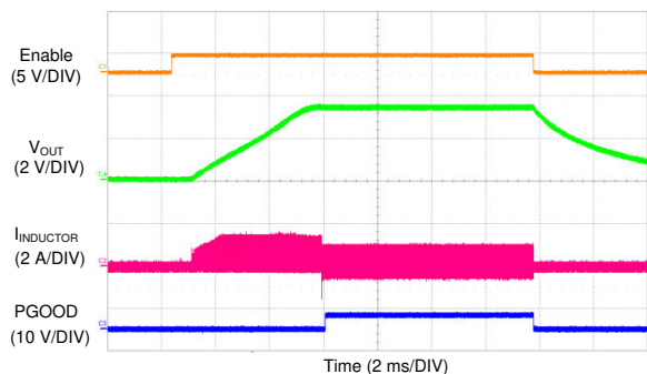
FIG 9-51. LM73606-Q1 Overcurrent Behavior
