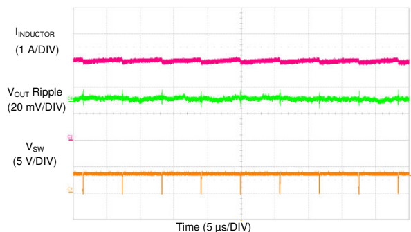
FIG 9-48. LM73606-Q1 Switching Waveform and V_{OUT} Ripple
