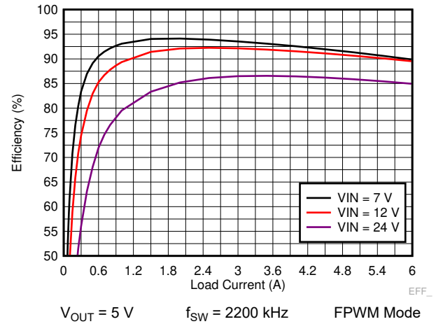
9-18. LM73606-Q1 Efficiency
