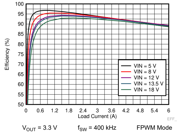
9-4. LM73606-Q1 Efficiency
