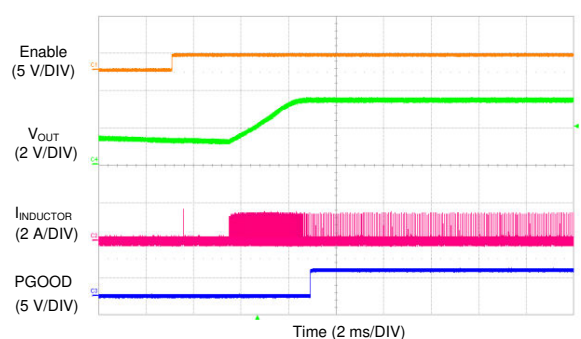
FIG 9-54. LM73606-Q1 Soft Start With 200-mA Load in Auto Mode
