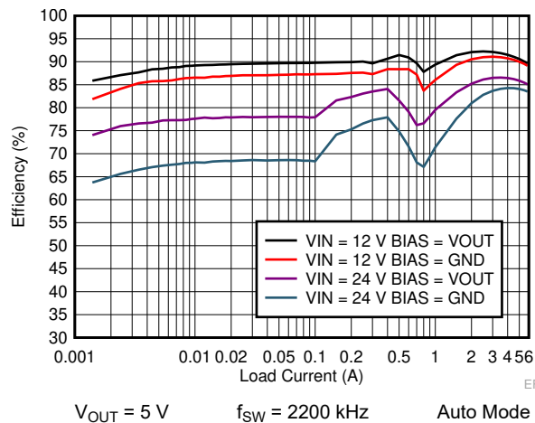
☒ 8-6. LM73606-Q1 Efficiency Comparison With Bias = V_{\text{OUT}} to Bias = GND in Auto Mode
