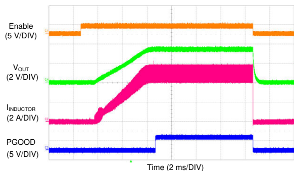
FIG 9-53. LM73606-Q1 Soft Start With 200-mA Load in FPWM Mode
