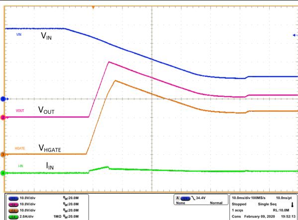
10-19. Overvoltage Recovery
