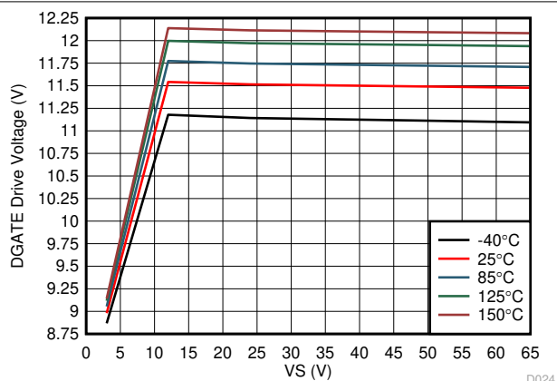
7-5. DGATE Drive Voltage vs Supply Voltage
