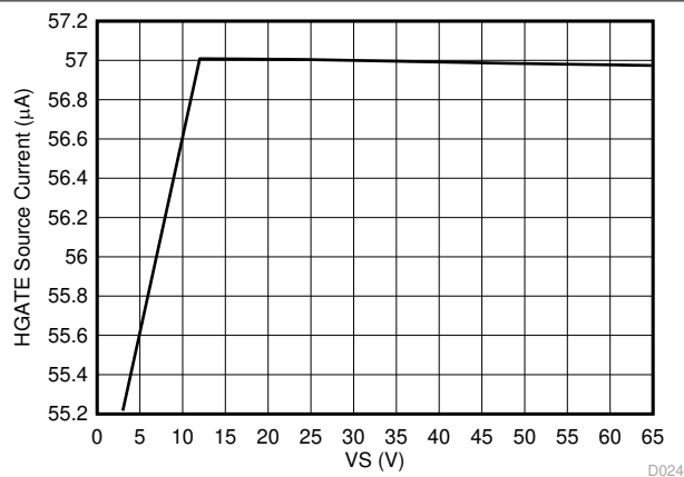
7-14. HGATE Current ( I_{HGATE} ) vs Supply Voltage
