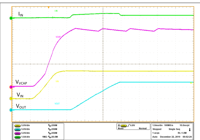
10-8. Startup 12 V showing Charge Pump VCAP
