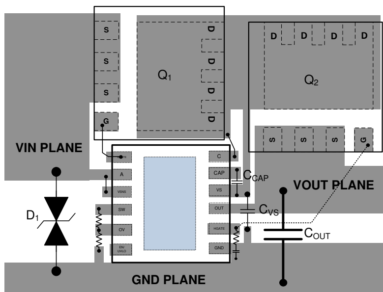
FIG 12-1. PCB Layout Example for Common Drain Configuration
