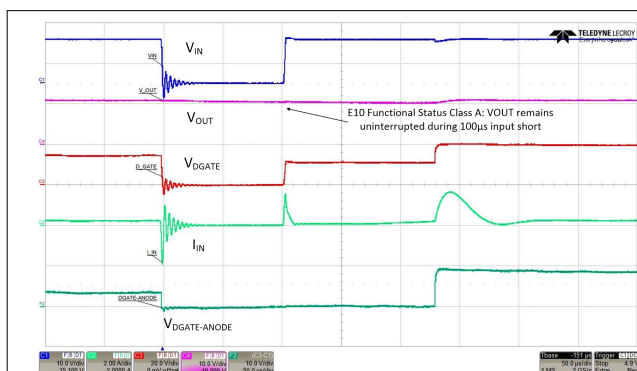
Figure 10-5. Input Micro-Short - LV124 E10 TC 2 100 \mu s
