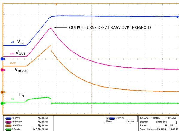
10-18. Overvoltage Protection
