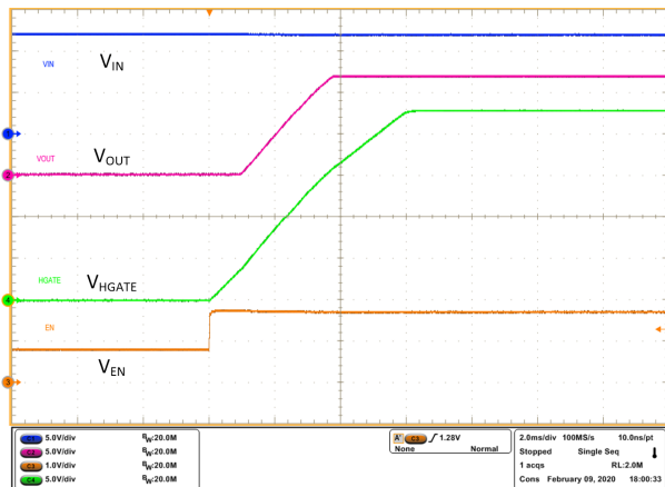
10-16. Turn ON with VCAP ON - EN rising from 0.8 V
