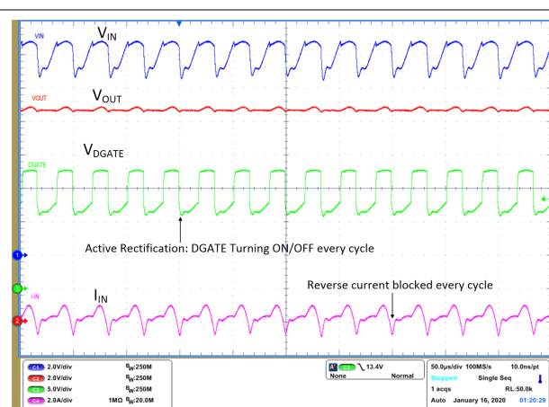
Figure 10-4. AC Super Imposed Test - 2-V Peak-Peak 30 KHz
