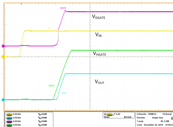
10-33. Power up 12 V - DGATE and HGATE
