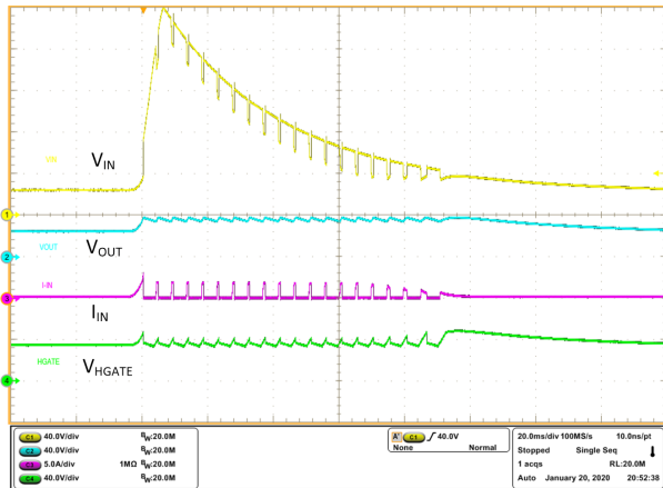
10-26. Unsuppressed Load Dump 200 V - Output Clamp
