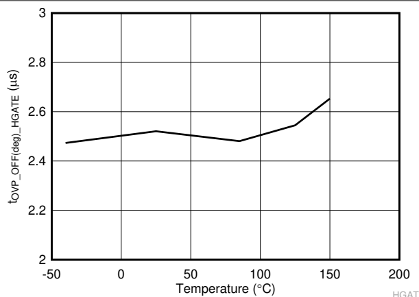
7-13. HGATE Turn OFF Delay during OV
