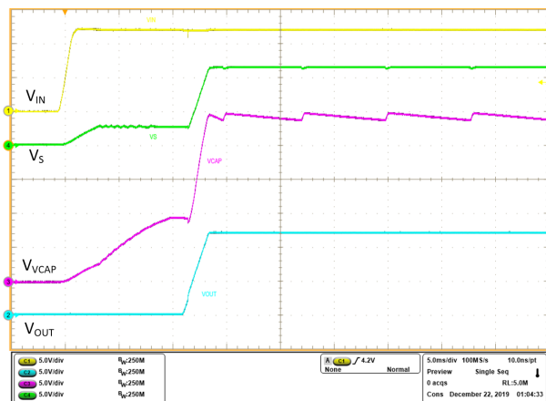
10-32. Power up 12 V - Charge Pump VCAP
