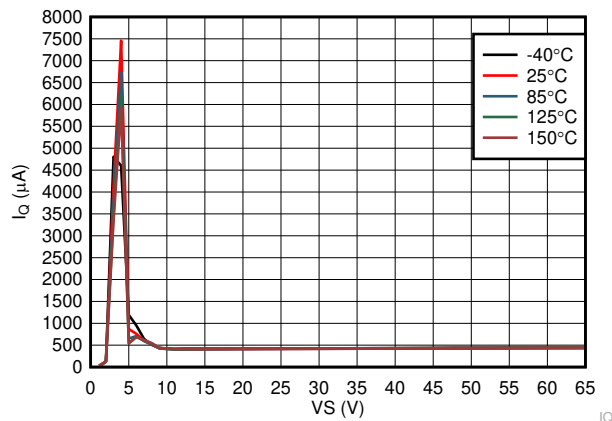
7-1. Operating Quiescent Current vs Supply Voltage
