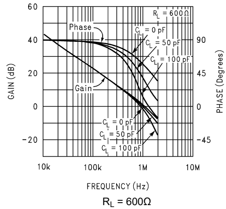
FIG 5-14. Gain and Phase Response vs Capacitive Load
