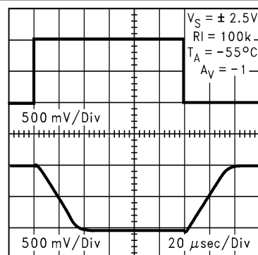
图 5-34. Inverting Large-Signal Pulse Response at 5V
