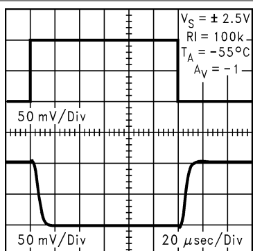
图 5-31. Inverting Small-Signal Pulse Response at 5V
