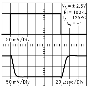
图 5-33. Inverting Small-Signal Pulse Response at 5V
