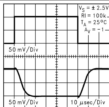
图 5-32. Inverting Small-Signal Pulse Response at 5V
