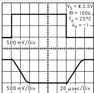
图 5-35. Inverting Large-Signal Pulse Response at 5V
