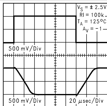
图 5-36. Inverting Large-Signal Pulse Response at 5V
