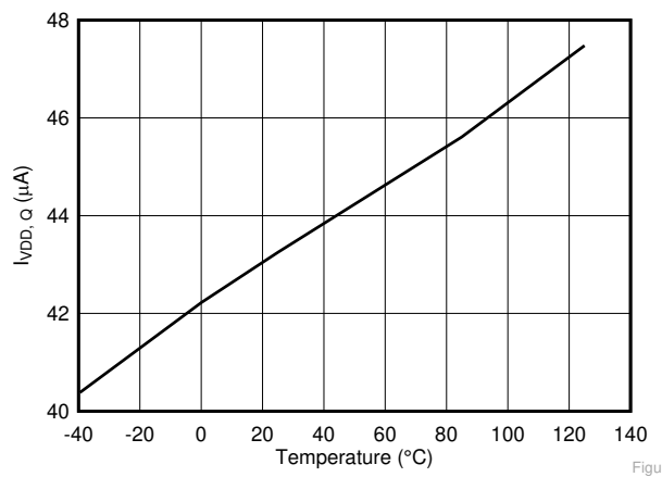
5-3. Quiescent Current
