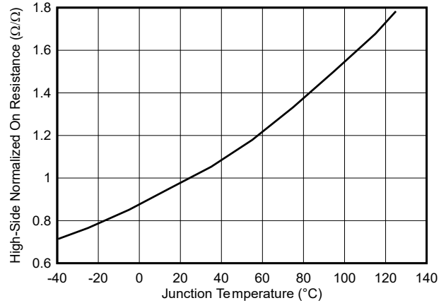
5-2. High-Side Normalized On-Resistance vs Junction Temperature
