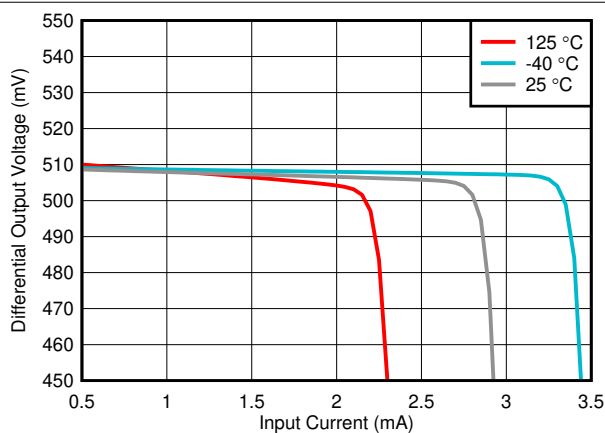
FIG 6-40. Low-side Swing vs Input Current
