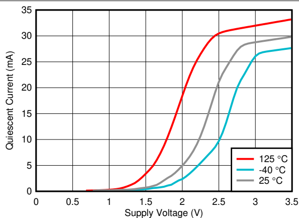
FIG 6-38. Quiescent Current vs Supply Voltage
