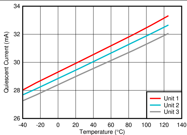
FIG 6-37. Quiescent Current vs Ambient Temperature
