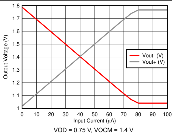
FIG 6-39. High-side Swing vs Input Current
