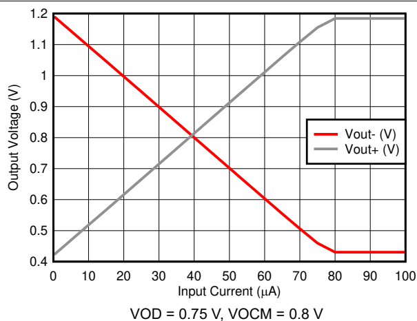
FIG 6-40. Low-side Swing vs Input Current
