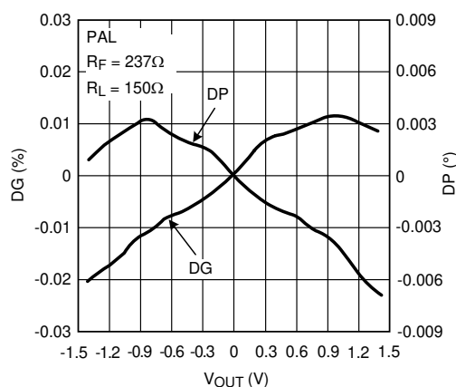
FIG 5-18. DG/DP (PAL)
