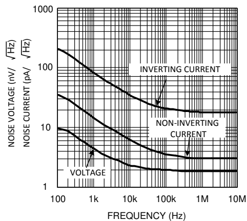
FIG 5-14. Noise
