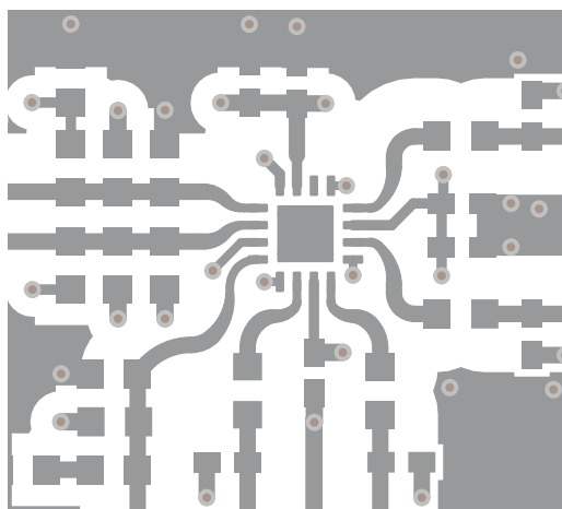
✕ 16. General PCB Ground Layout for Thermal Reliability
