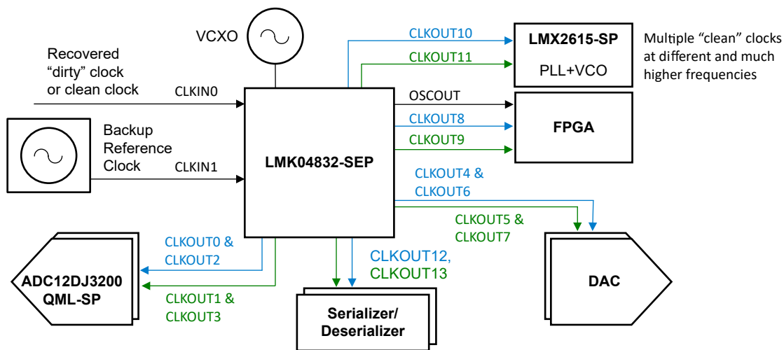
9-6. Typical Application
