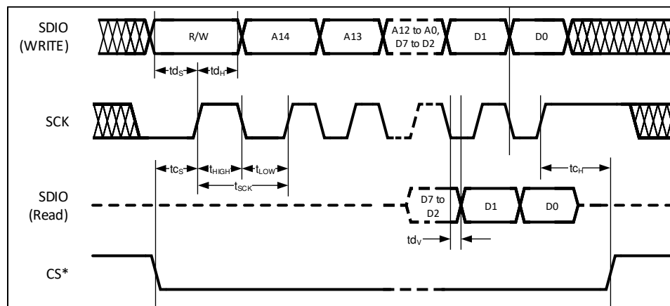
6-1. SPI Timing Diagram
