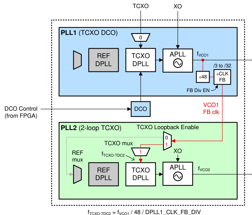
図 7-37. PLL Cascading Example With DCO Frequency Steering
