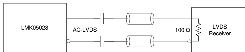
✎ 7-30. AC-LVDS Output to LVDS Receiver With Internal Termination/Biasing
