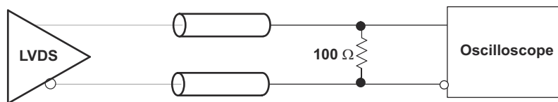
FIG 7-1. LVDS Output DC Configuration During Device Test
