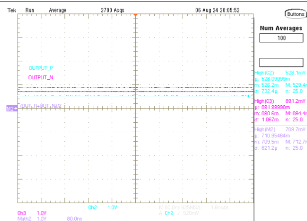
図 6-11. LMK1D210xL DC Output Common Mode at 1.8V Supply Condition, Differential Low (AMP_SELA / AMP_SELB = 0)
