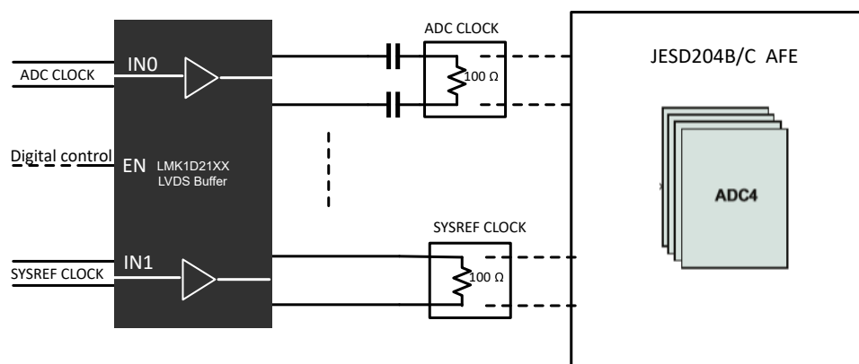
FIG 9-1. Fan-Out Buffer for ADC Device Clock and SYSREF Distribution
