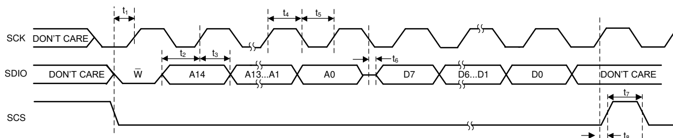
图 6-3. SPI 3-Wire Read Timing Diagram
