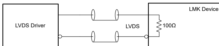
図 8-12. DC-Coupled HSDS/LVDS to Reference (INx)
