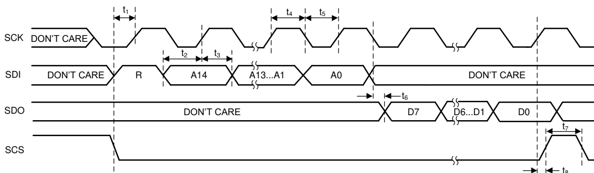
图 6-2. SPI 4-Wire Read Timing Diagram
