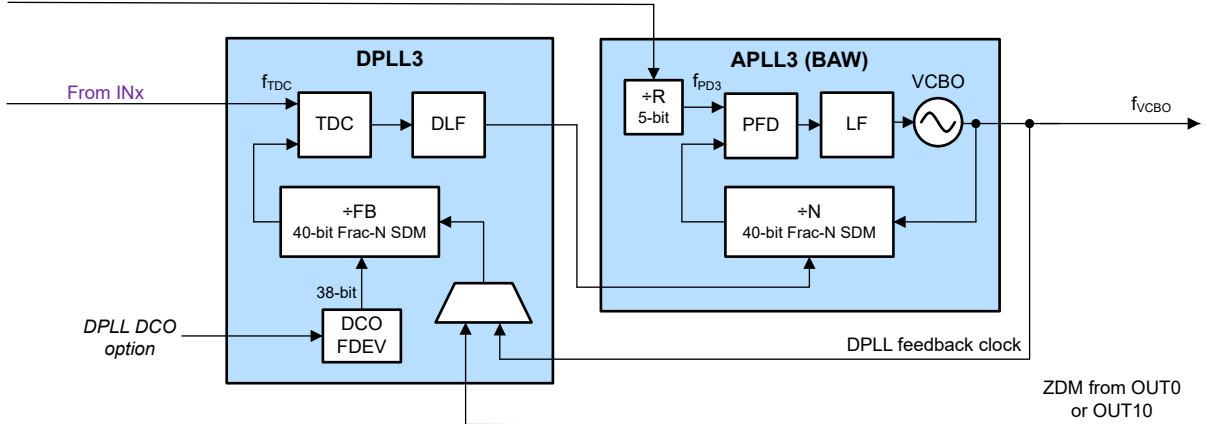
图 8-5. APLL Cascaded With DPLLs Enabled Example
