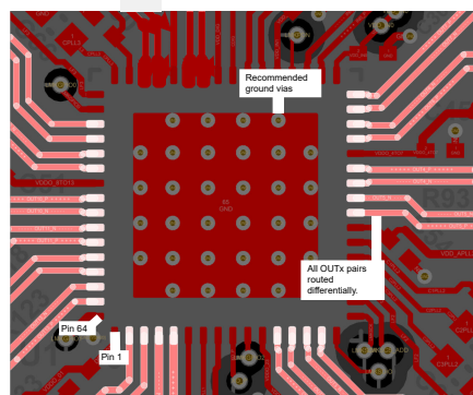
図 9-5. PCB Layout Example for LMK5B33414, Top Layer
