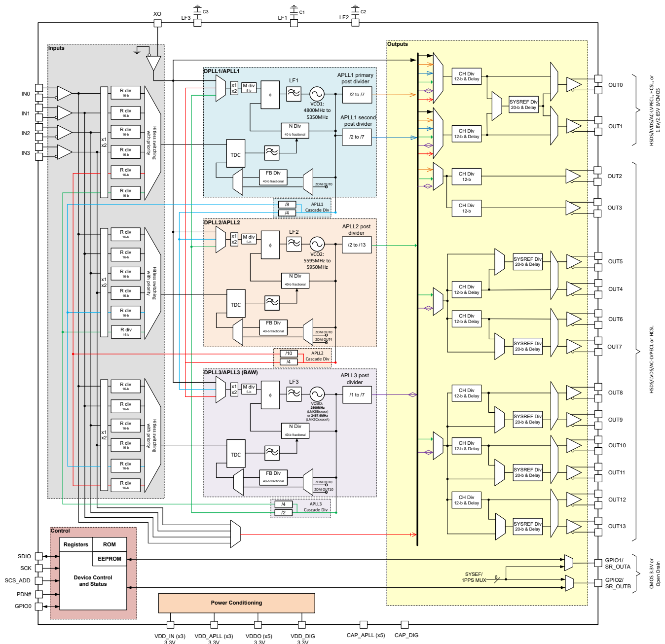
図 8-1. LMK5B33414 Top-Level Block Diagram
