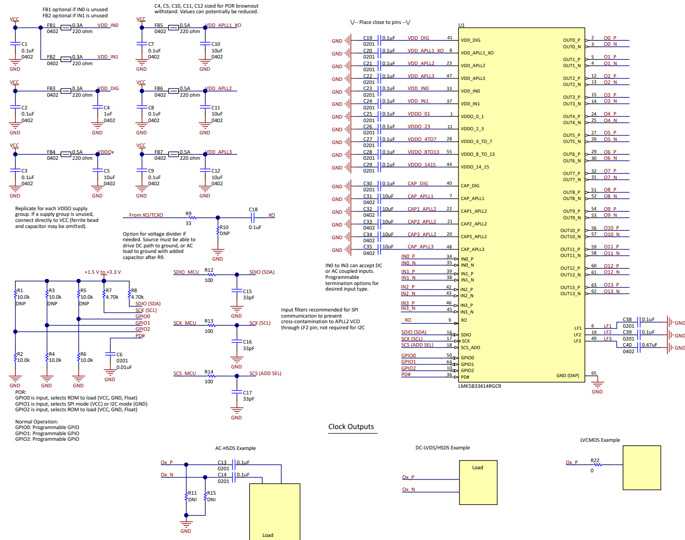
9-3. Typical Application Example
