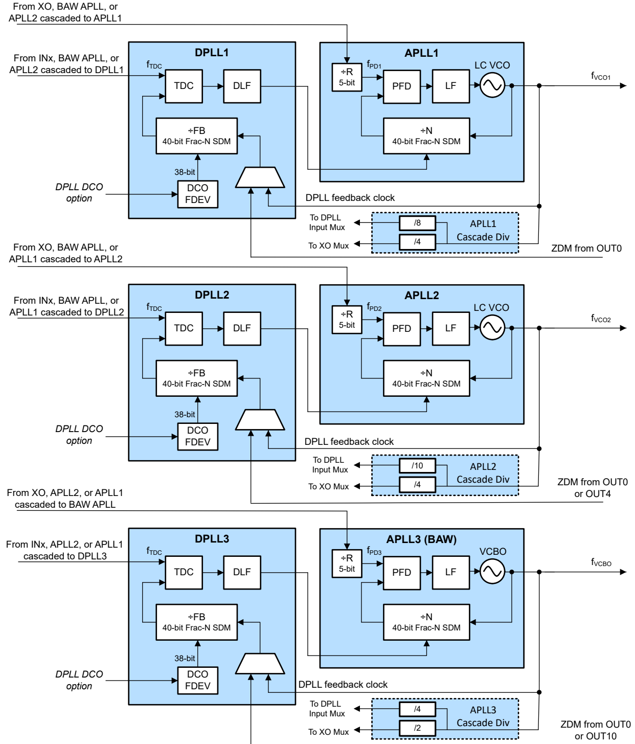
図 8-2. PLL Architecture
