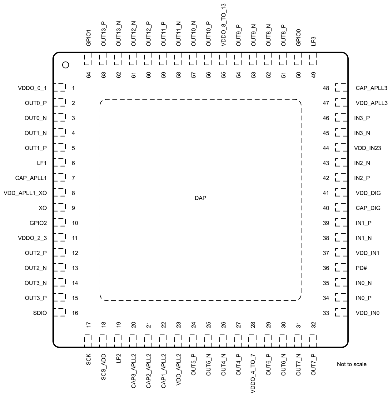
図 5-1. LMK5B33414 RGC Package 64-Pin VQFN Top View
