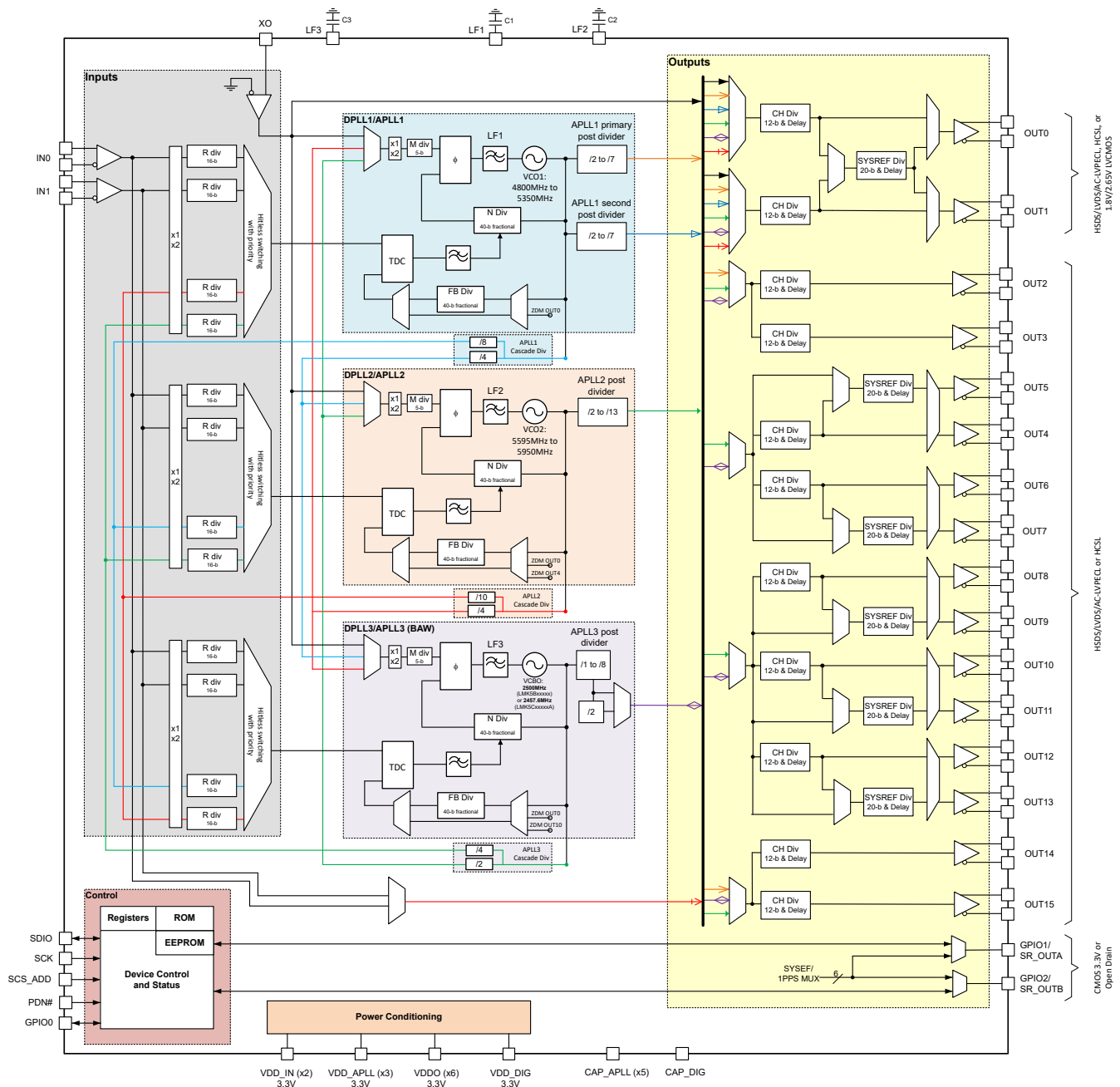
図 8-1. LMK5C33216A Top-Level Block Diagram
