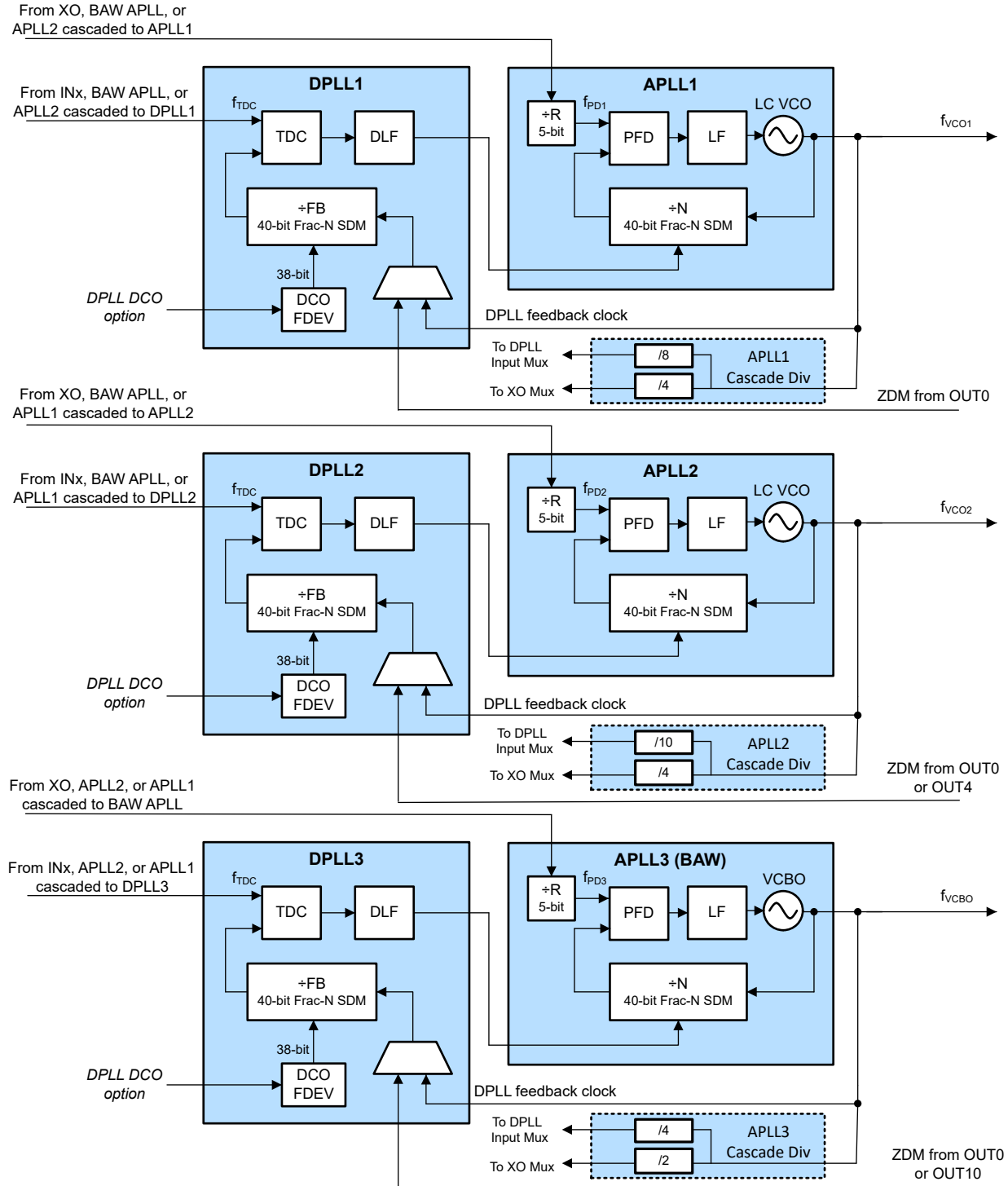
図 8-2. PLL Architecture
