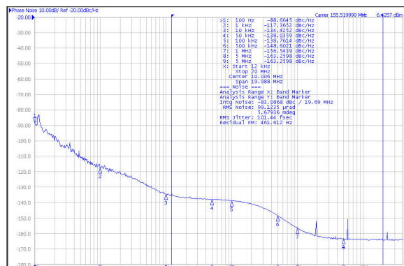
図 6-15. 155.52MHz HSDS Output From APLL2
