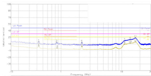
V_{IN} = 12.5V V_{OUT} = 3.3V F_{sw} = 2.2MHz 負荷 = 3A
