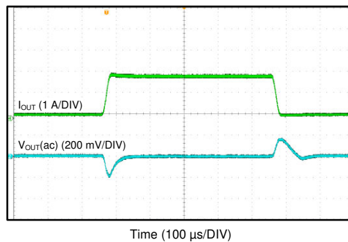
7-5. DCM Mode
