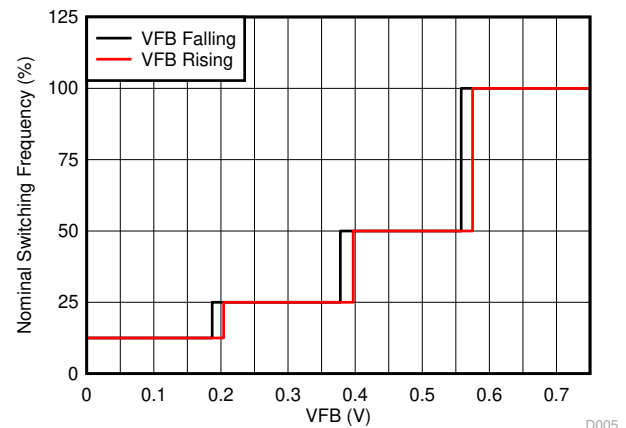
Figure 5-6. Frequency vs V_{FB}
