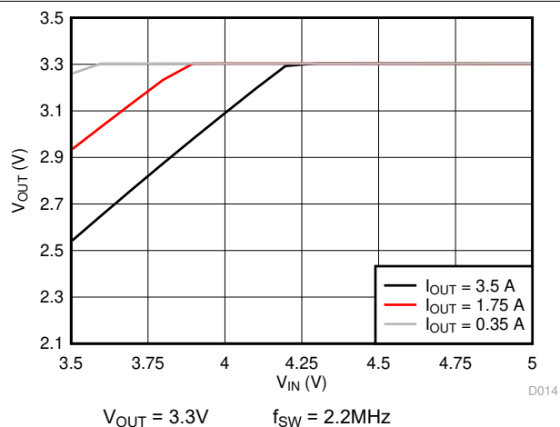
图 5-10. Dropout Curve
