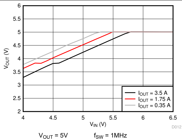
图 5-8. Dropout Curve
