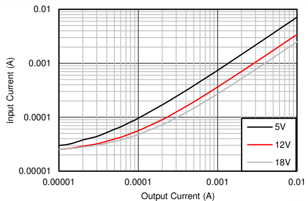
FIG 8-5. Input Supply Current vs Output Current for 3.3-V Fixed Output Option
