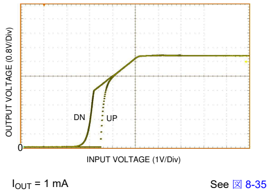
Figure 6-5. UVLO Thresholds
