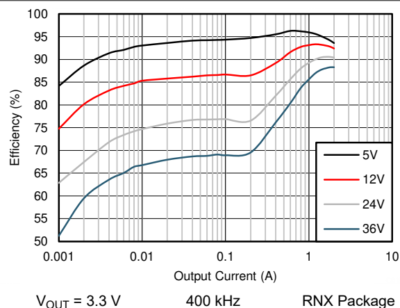
Figure 8-12. Efficiency
