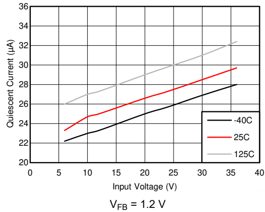
Figure 6-1. Non-Switching Input Supply Current
