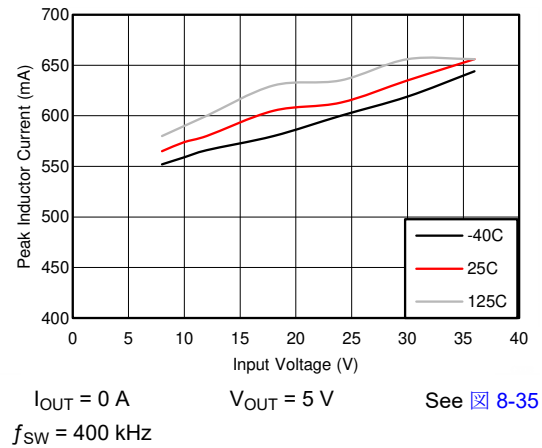
Figure 6-6. I_{PEAK-MIN}
