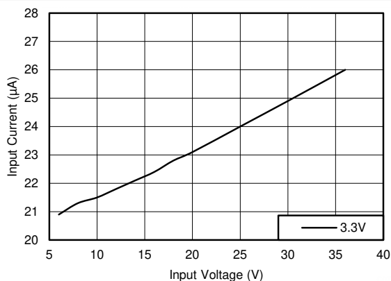
FIG 8-4. No-load Input Supply Current for 3.3-V Fixed Output Option
