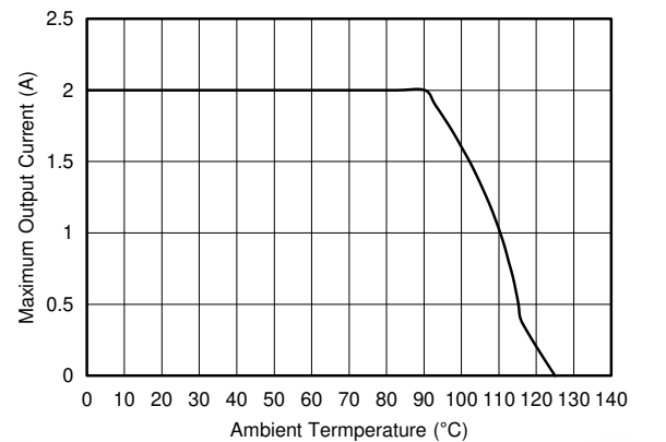
Figure 8-8. Maximum Output Current versus Ambient Temperature
