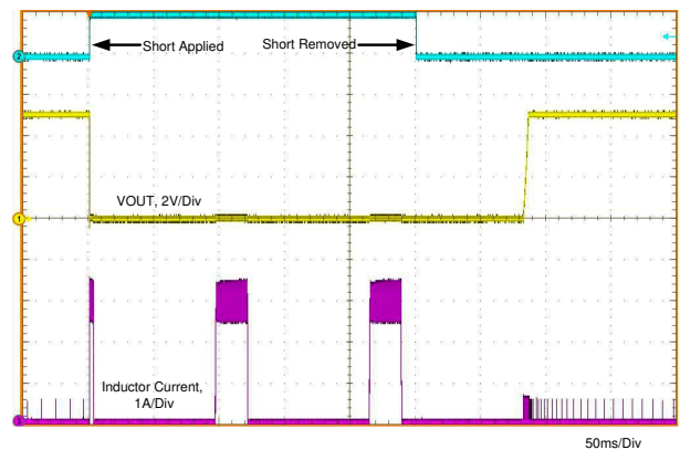
図 7-6. Short-Circuit Transient and Recovery
