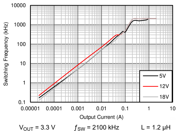
8-26. Switching Frequency versus Output Current
