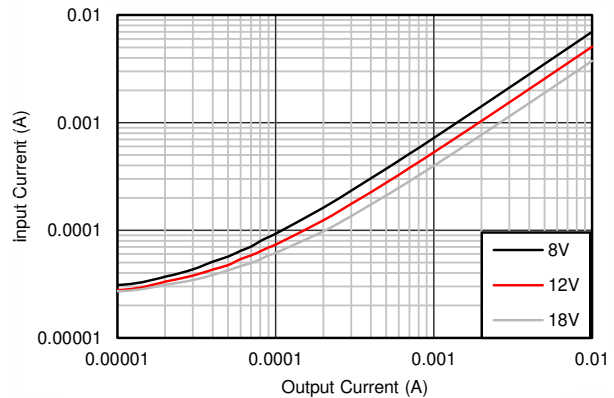
FIG 8-3. Input Supply Current vs Output Current for 5-V Fixed Output Option
