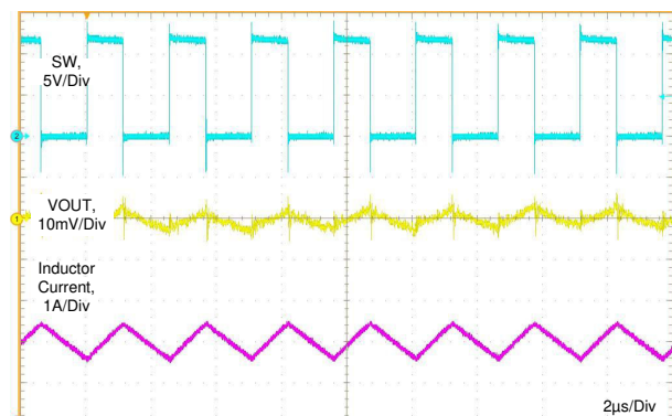
Figure 7-8. Typical PWM Switching Waveforms V_{IN} = 12 V, V_{OUT} = 5 V, I_{OUT} = 2 A, f_S = 400 kHz
