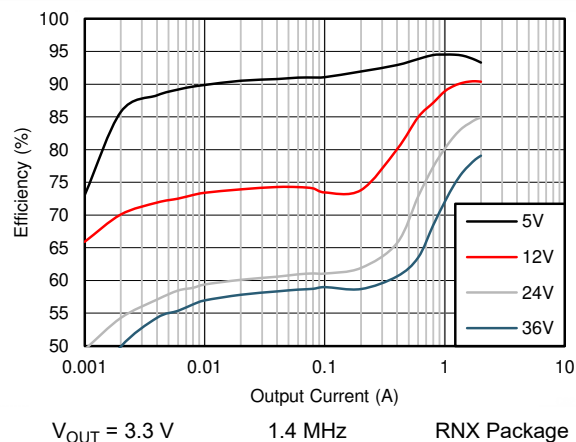
Figure 8-14. Efficiency
