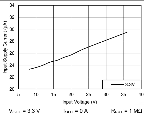
8-24. Input Supply Current
