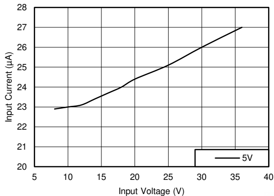
FIG 8-2. No-load Input Supply Current for 5-V Fixed Output Option
