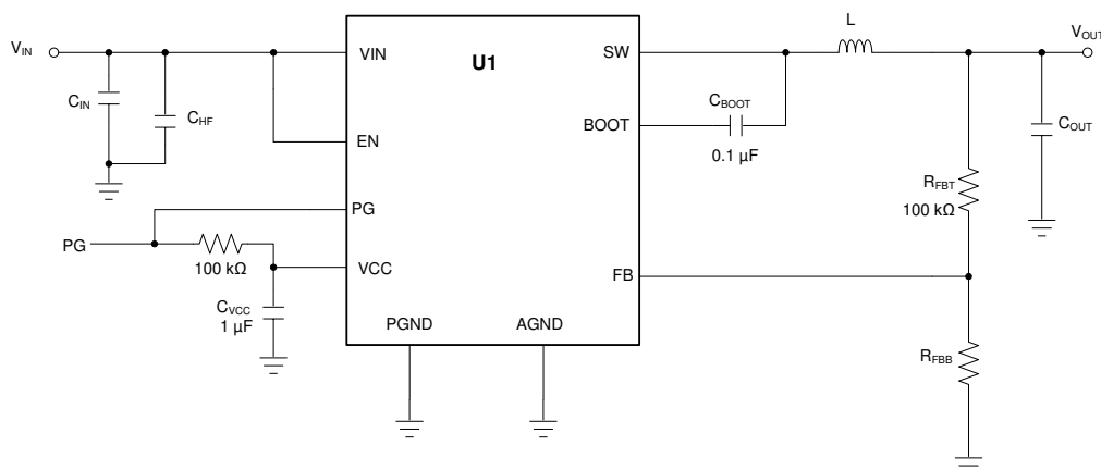
图 9-27. Circuit for Application Curves
