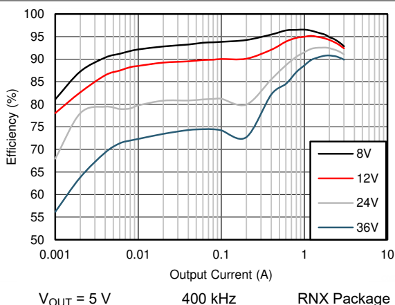
Figure 9-5. Efficiency
