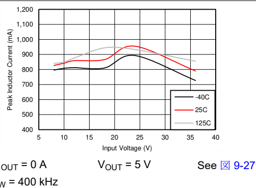
7-6. I_{PEAK-MIN}
