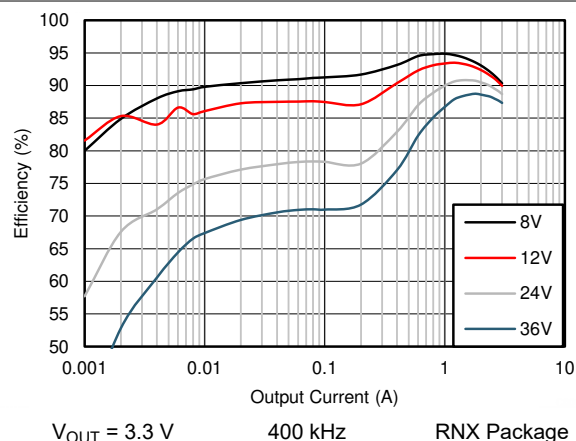
Figure 9-6. Efficiency
