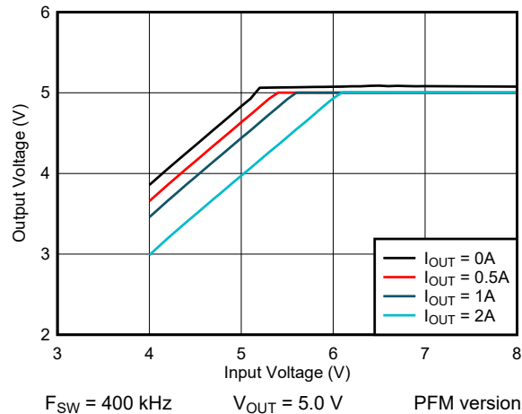
Figure 7-3. 5-V Dropout
