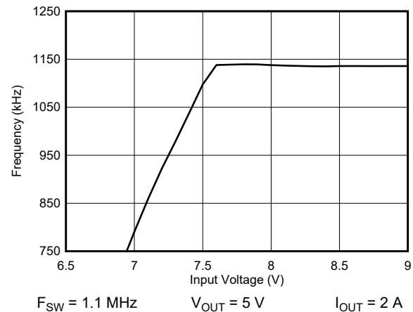
✎ 8-9. Typical Frequency Foldback at T_{OFF\_MIN}
