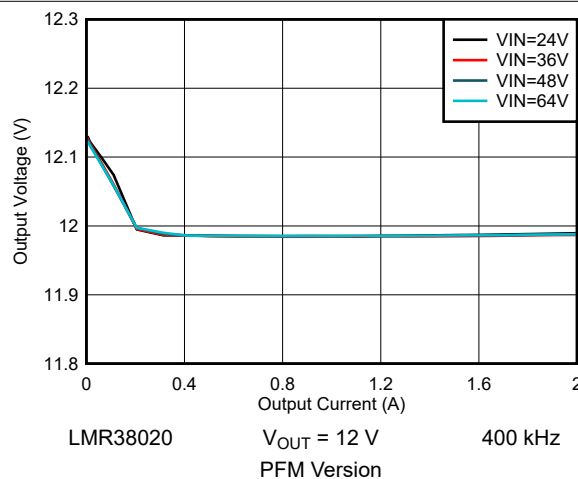
9-14. 12-V Load Regulation
