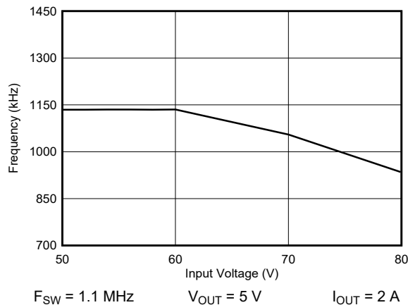
✎ 8-8. Typical Frequency Foldback at T_{ON\_MIN}
