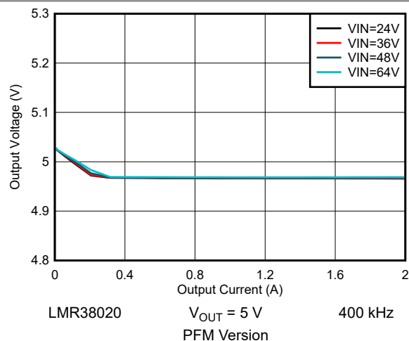
9-13. 5-V Load Regulation
